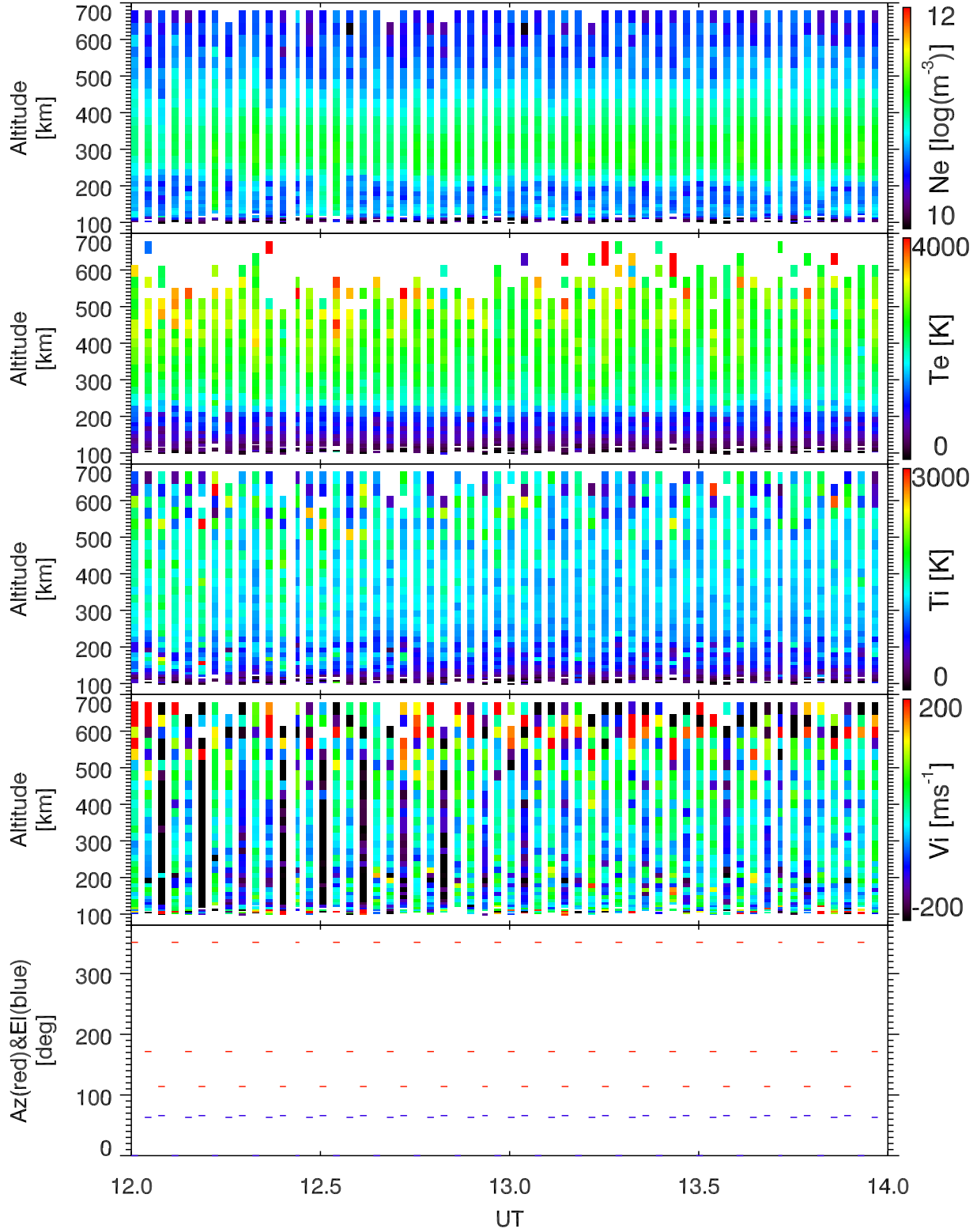
EISCAT 2002-11-01_12_14UT_tau0_ant@32m.
