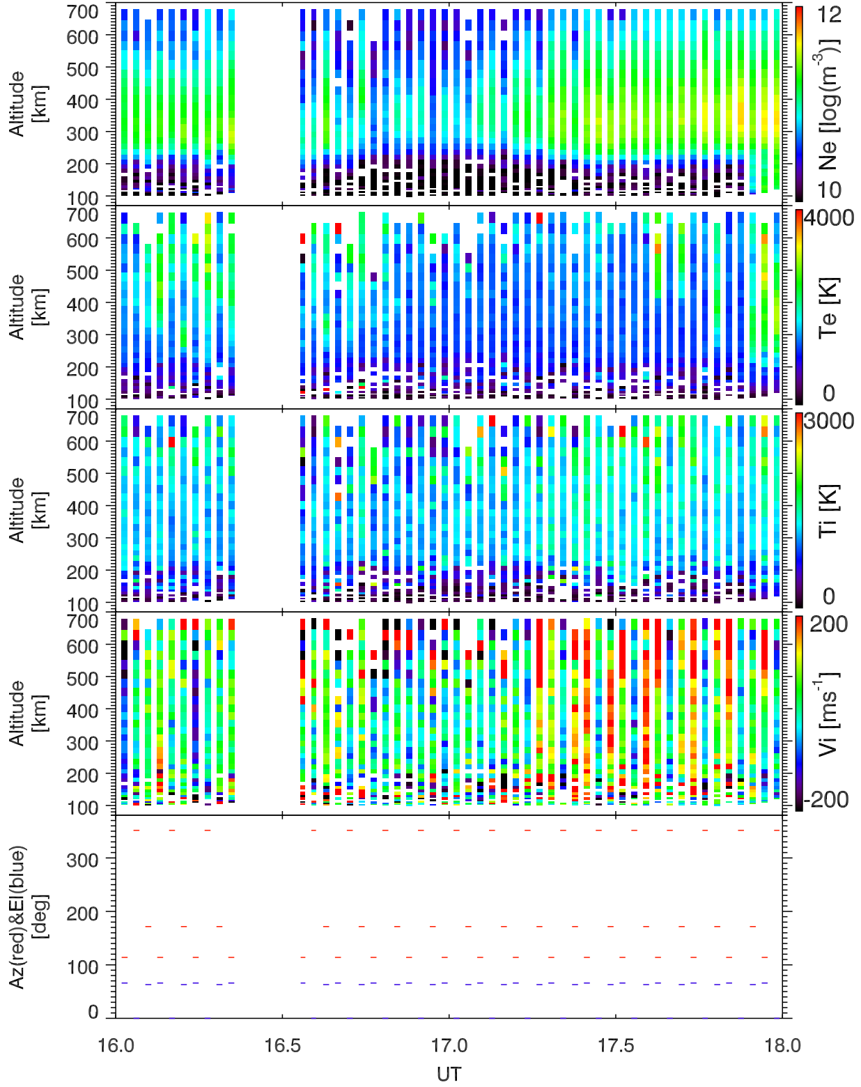
EISCAT 2002-11-01_16_18UT_tau0_ant@32m.
