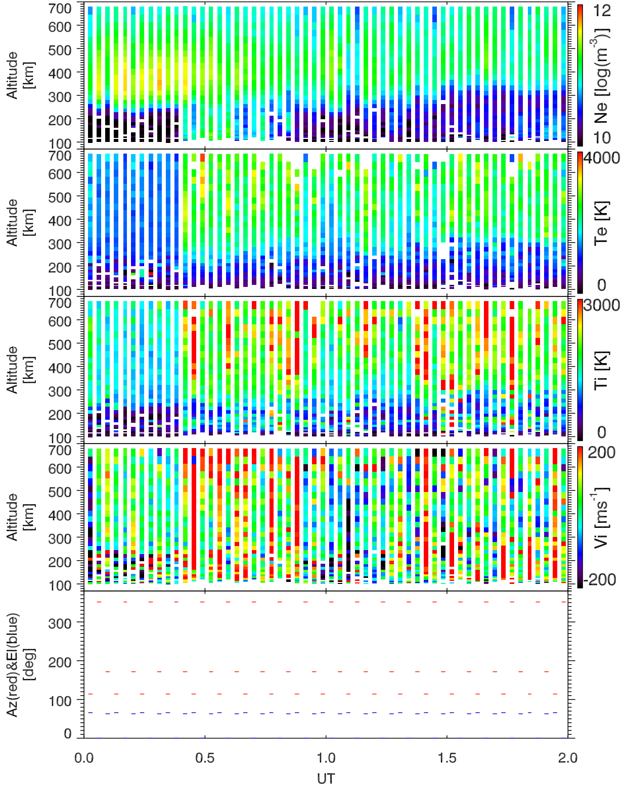
EISCAT 2002-11-02_00_02UT_tau0_ant@32m.
