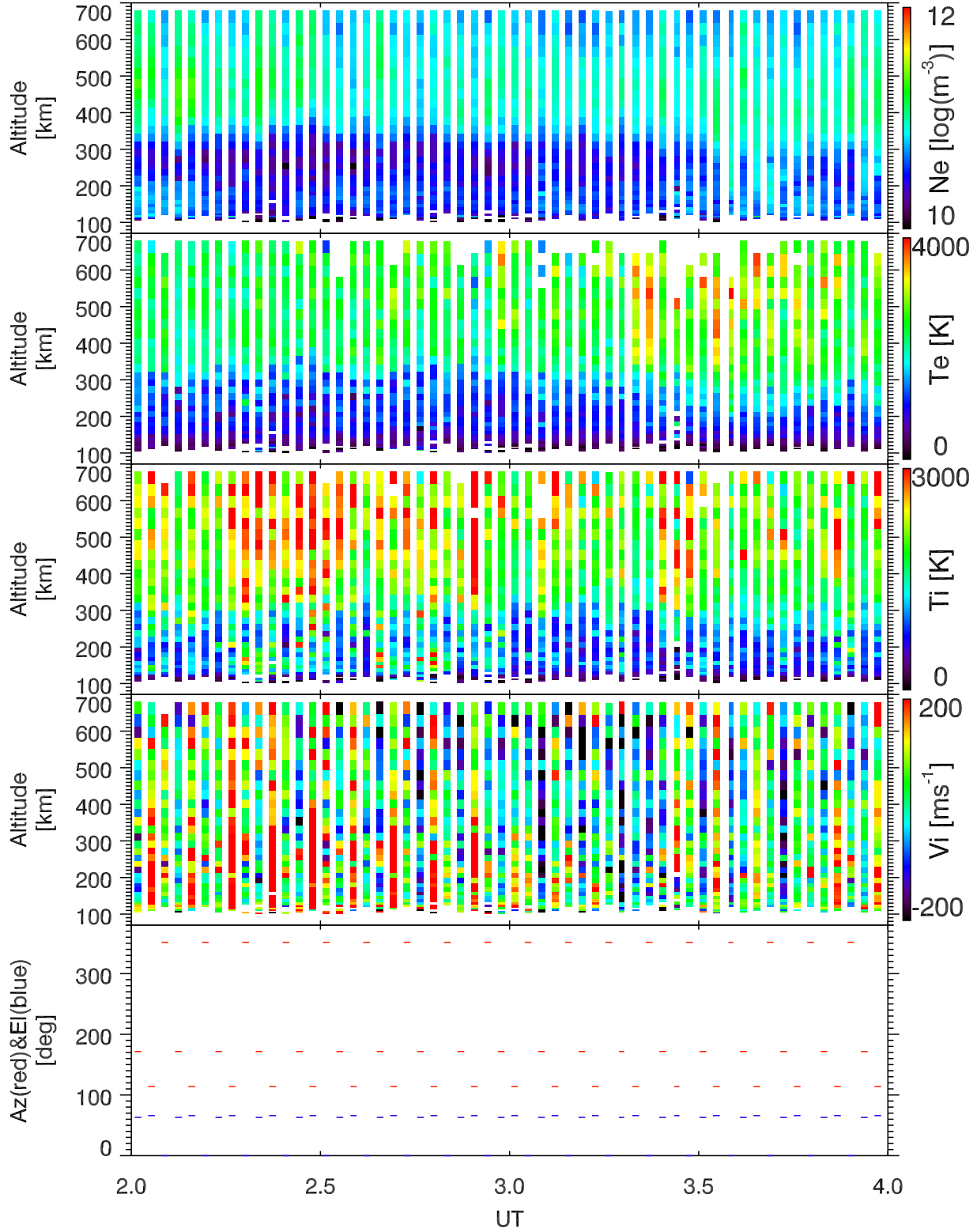
EISCAT 2002-11-02_02_04UT_tau0_ant@32m.
