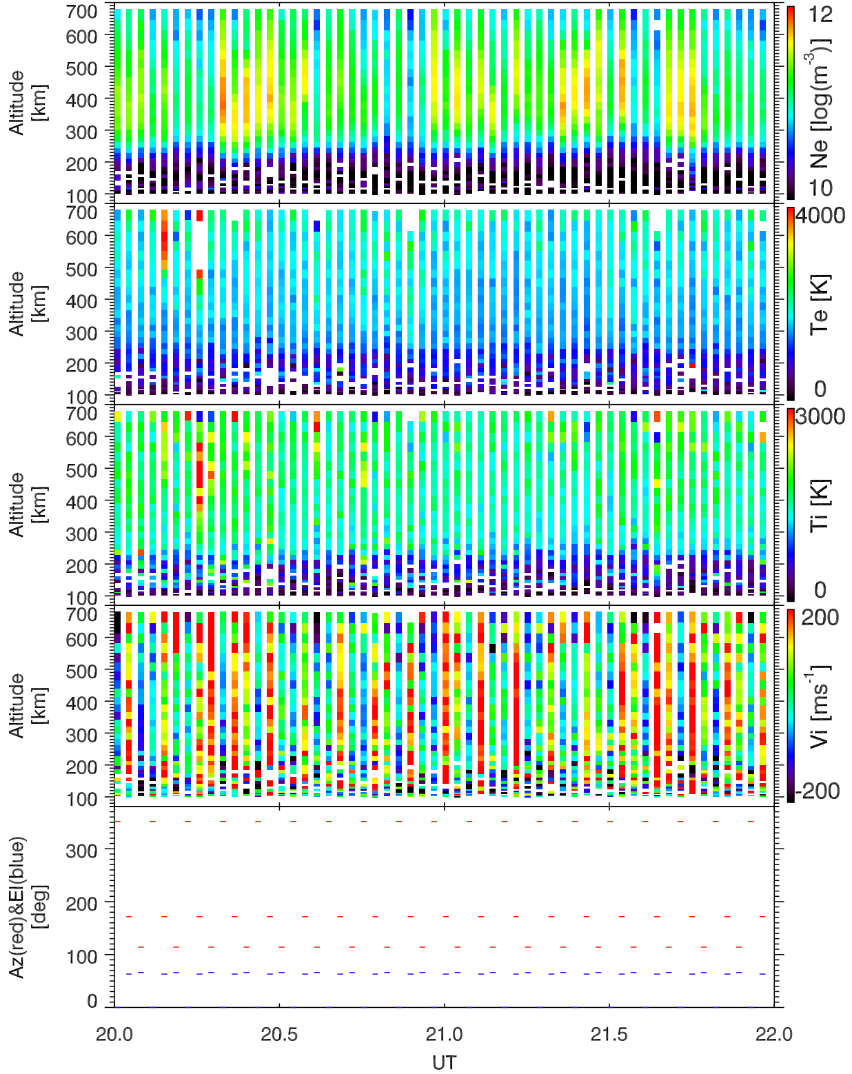
EISCAT 2002-11-02_20_22UT_tau0_ant@32m.
