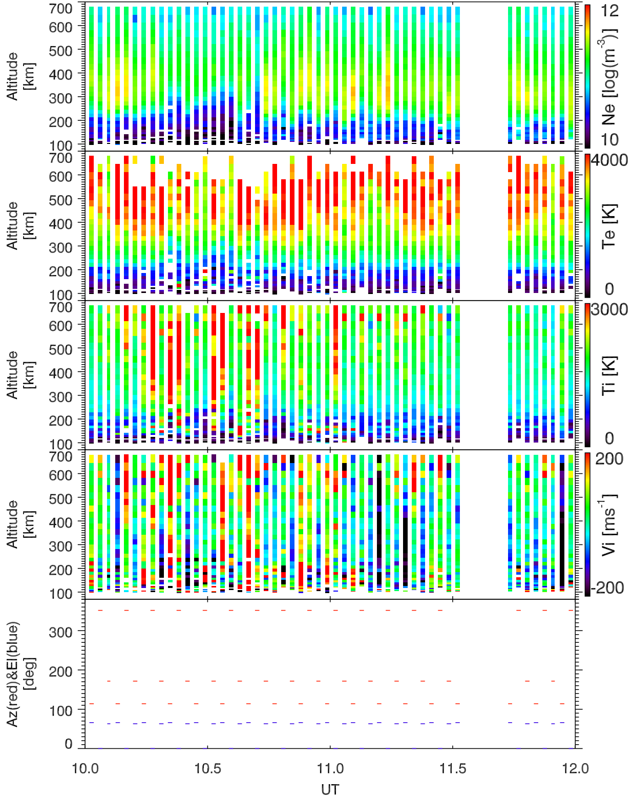
EISCAT 2002-11-11_10_12UT_tau0_ant@32m.
