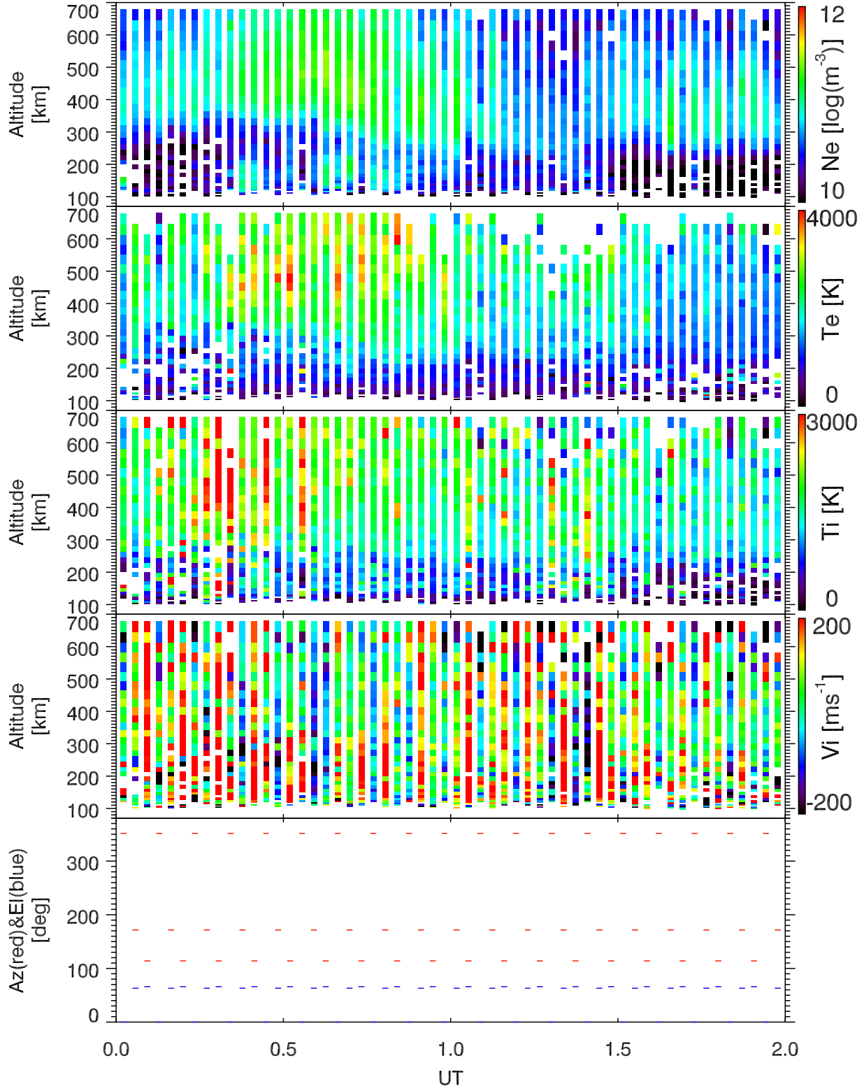
EISCAT 2002-11-13_00_02UT_tau0_ant@32m.
