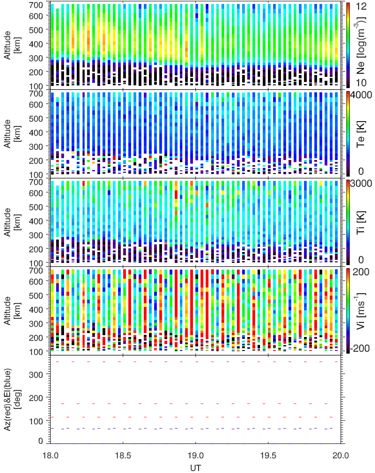
EISCAT 2002-11-14_18_20UT_tau0_ant@32m.
