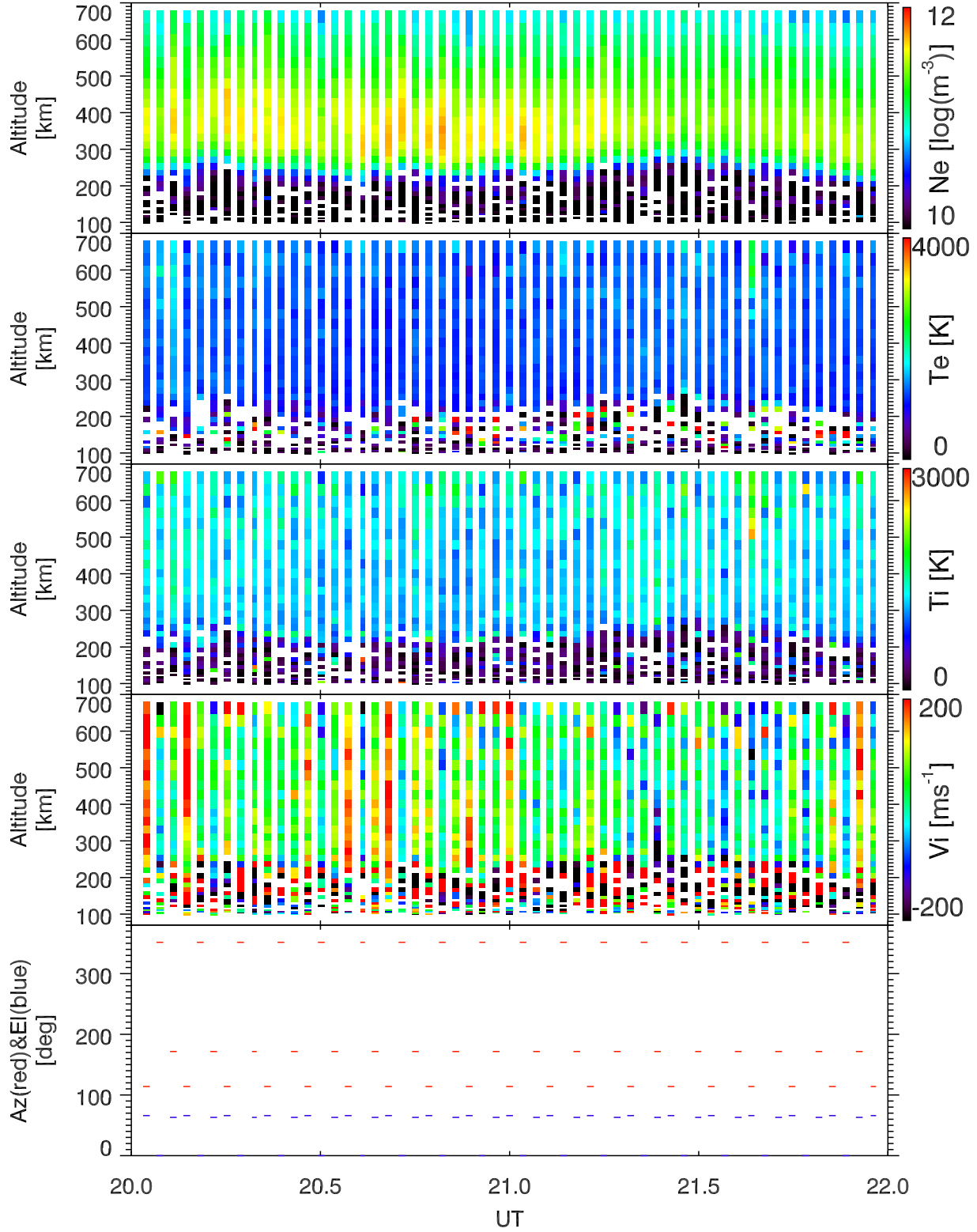
EISCAT 2002-11-14_20_22UT_tau0_ant@32m.
