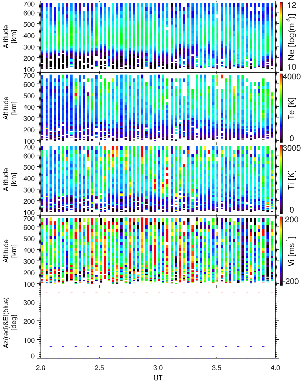
EISCAT 2002-11-15_02_04UT_tau0_ant@32m.
