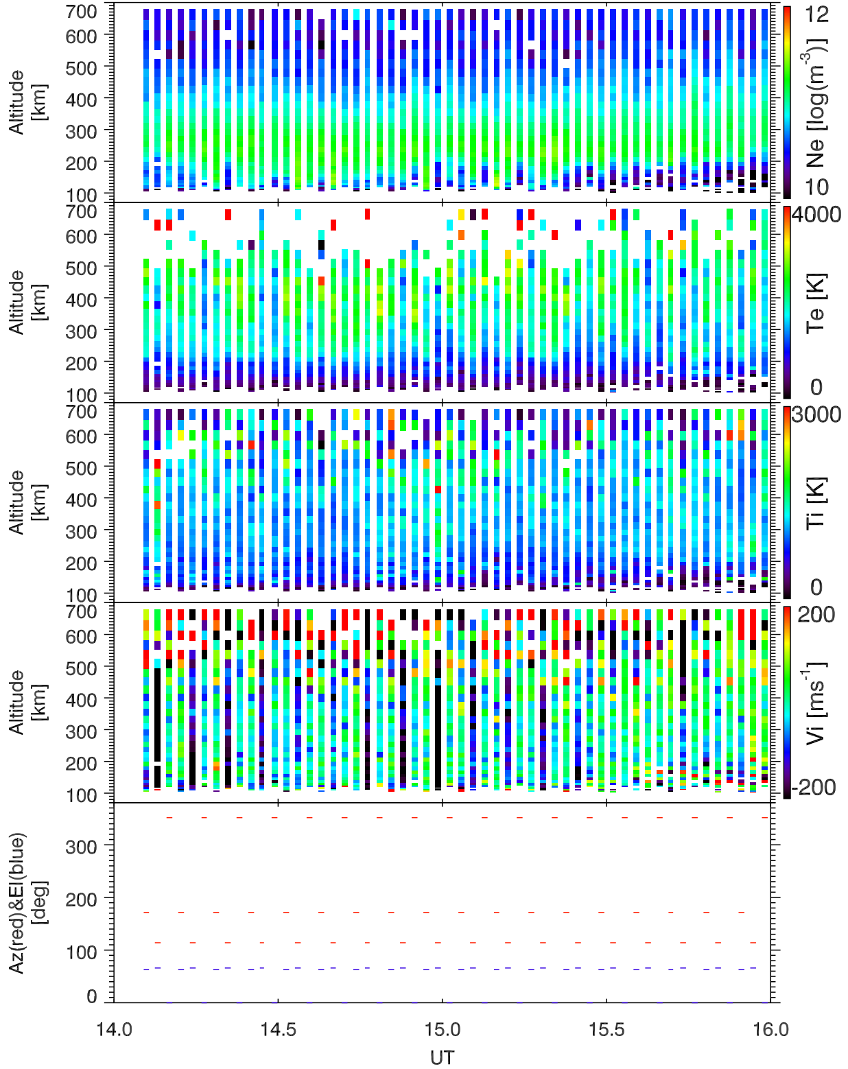
EISCAT 2003-01-07_14_16UT_tau0_ant@32m.
