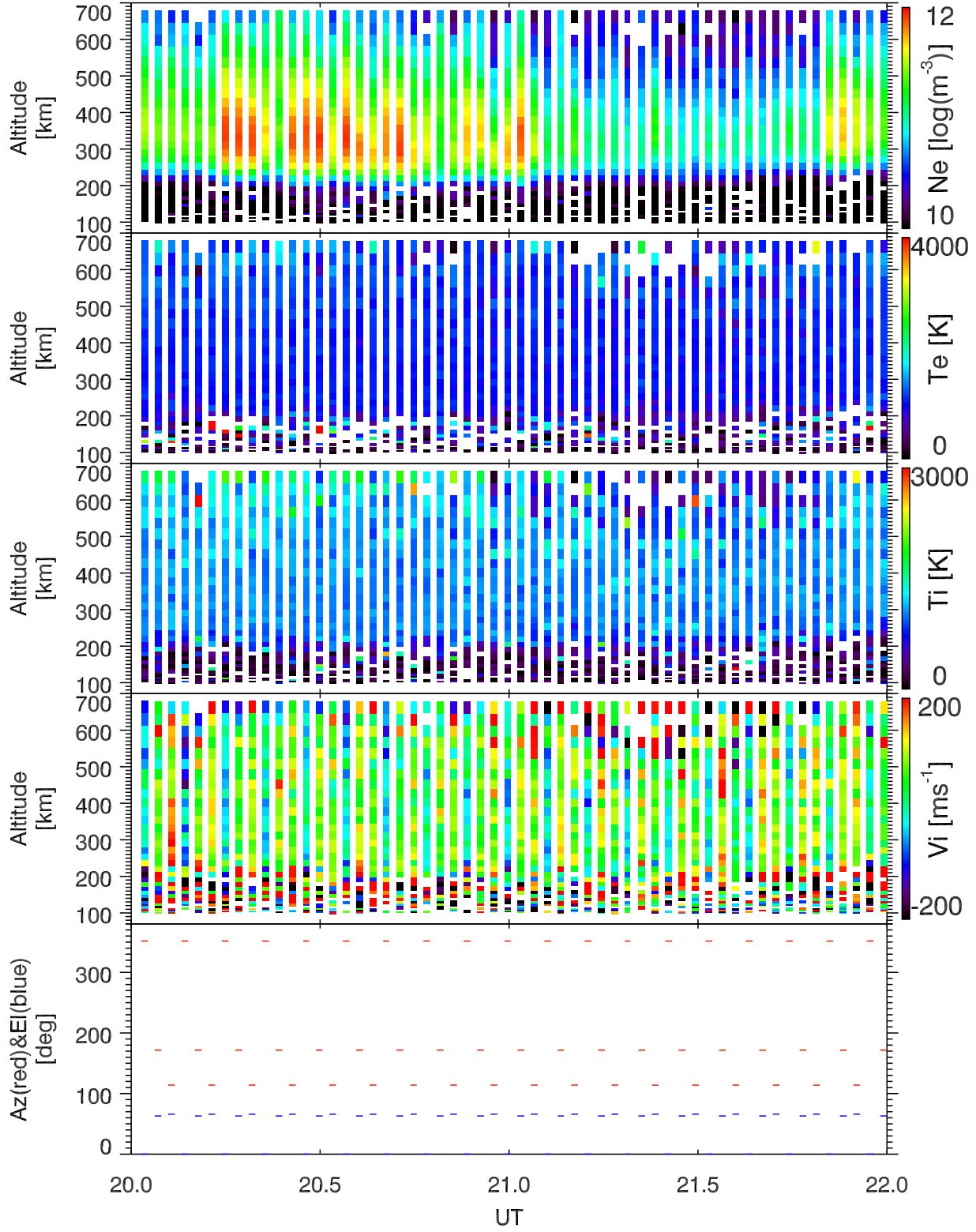
EISCAT 2003-01-07_20_22UT_tau0_ant@32m.
