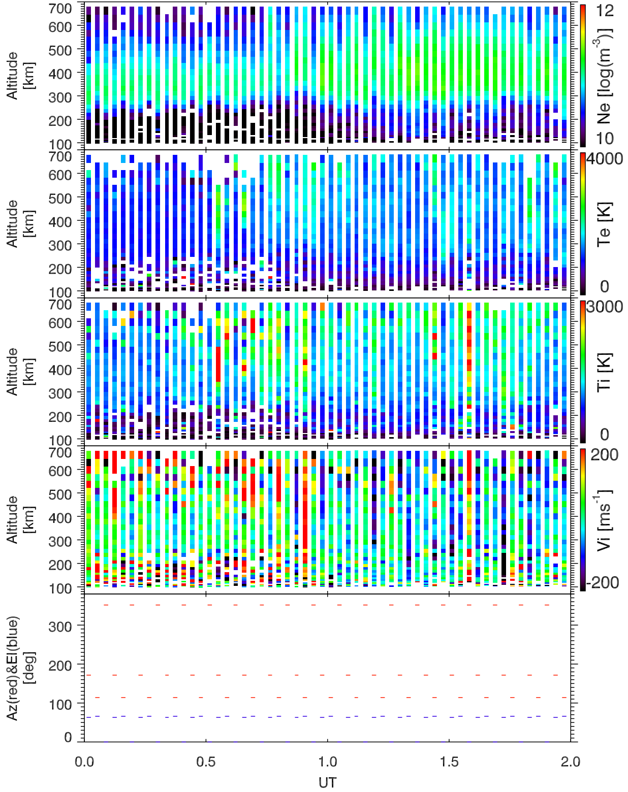
EISCAT 2003-01-08_00_02UT_tau0_ant@32m.
