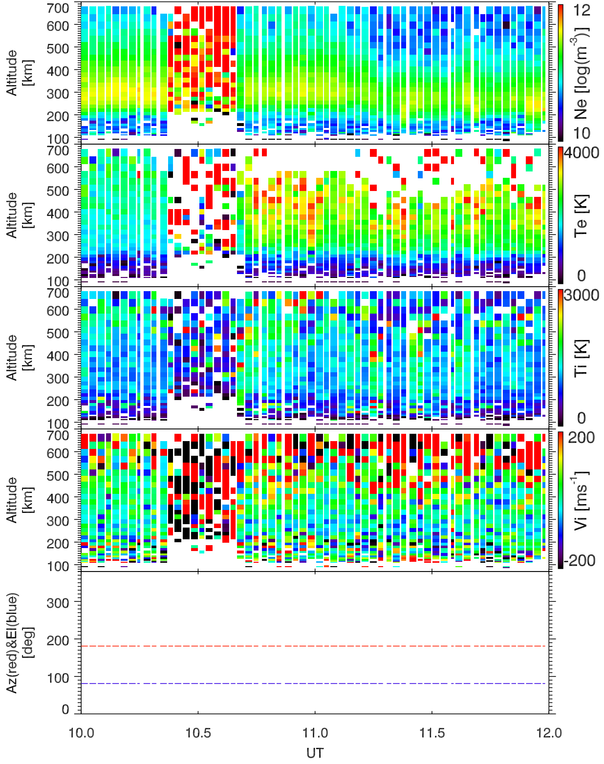
EISCAT 2003-02-24_10_12UT_tau0_120@42m.
