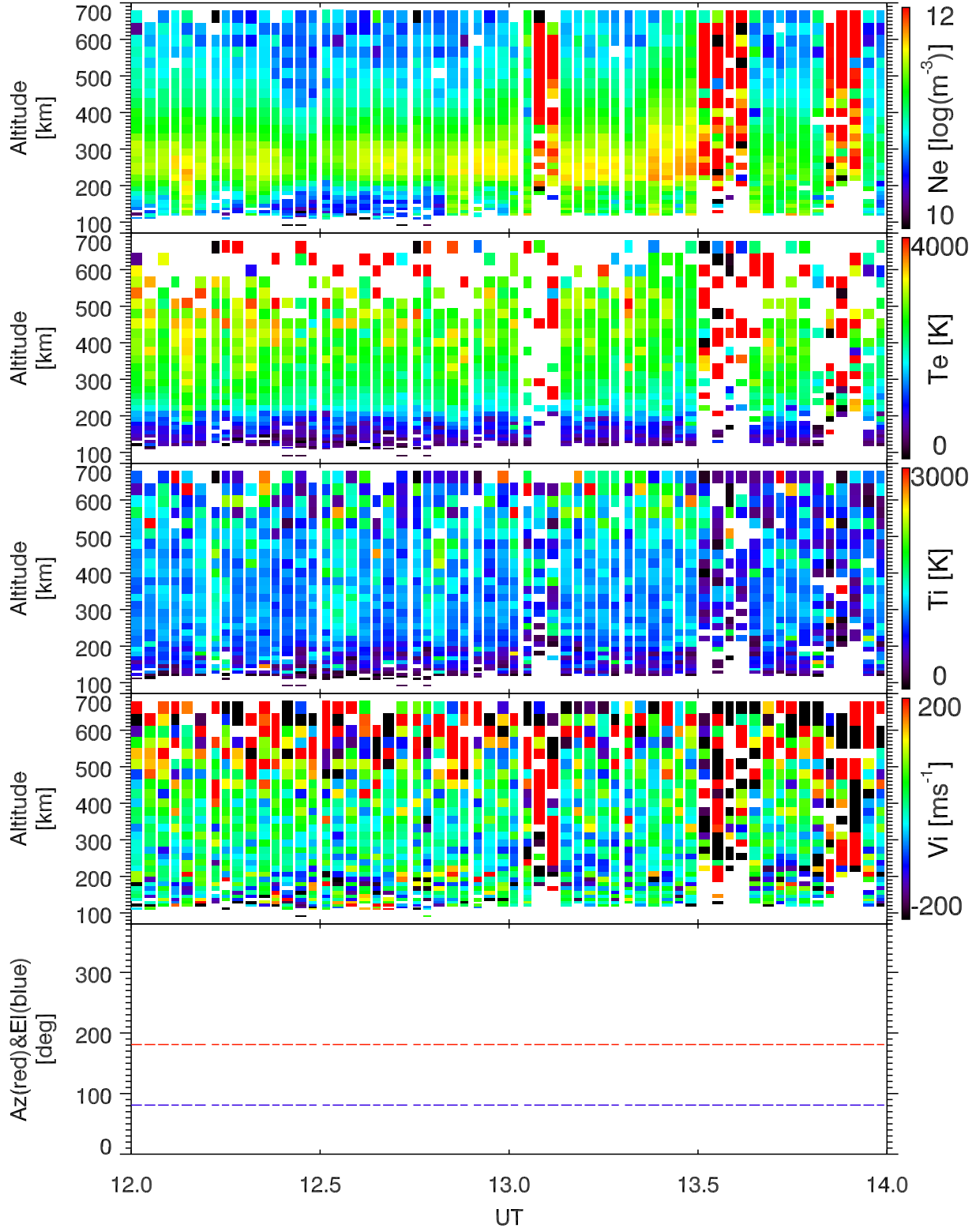
EISCAT 2003-02-24_12_14UT_tau0_120@42m.
