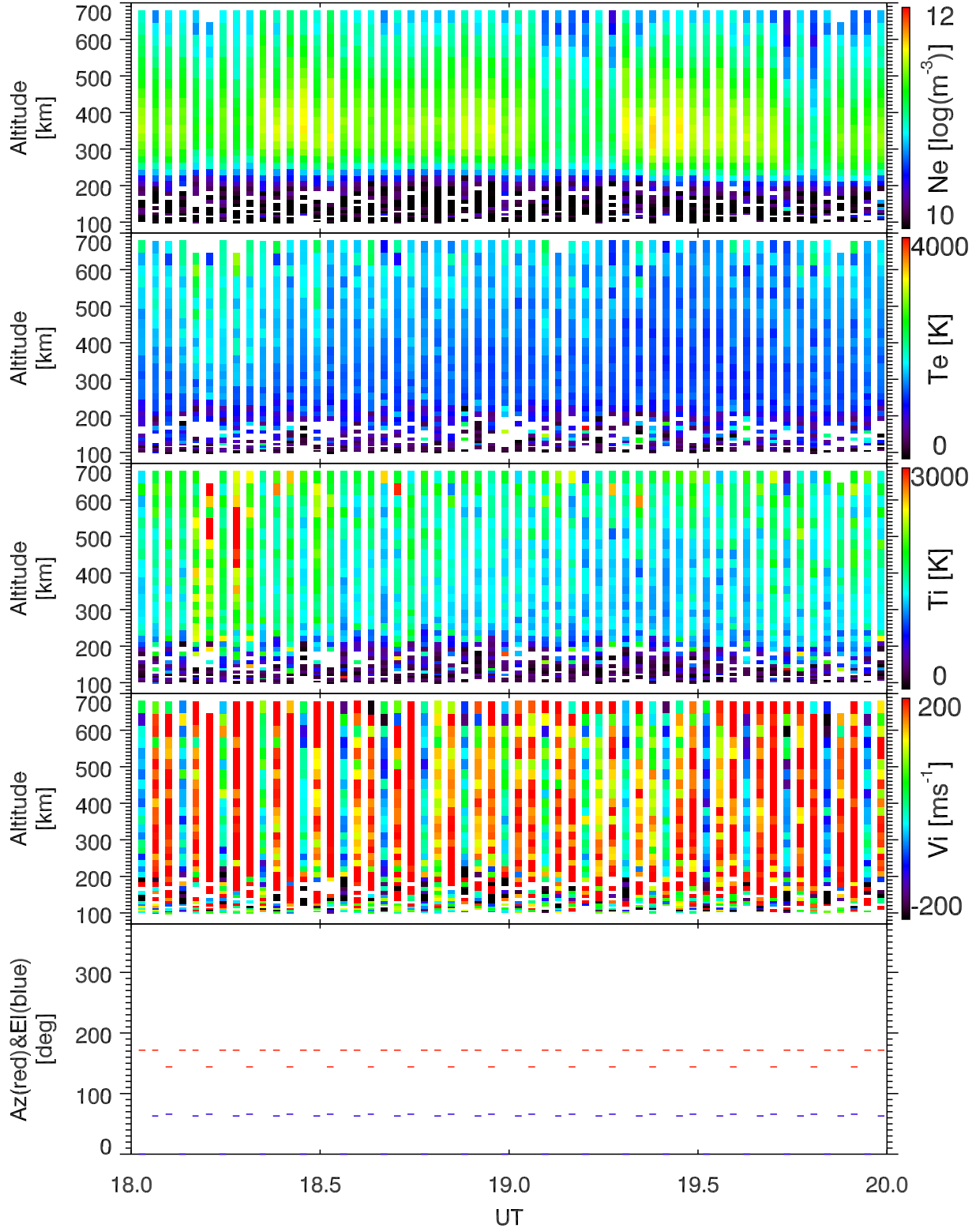
EISCAT 2003-02-28_18_20UT_tau0_ant@32m.
