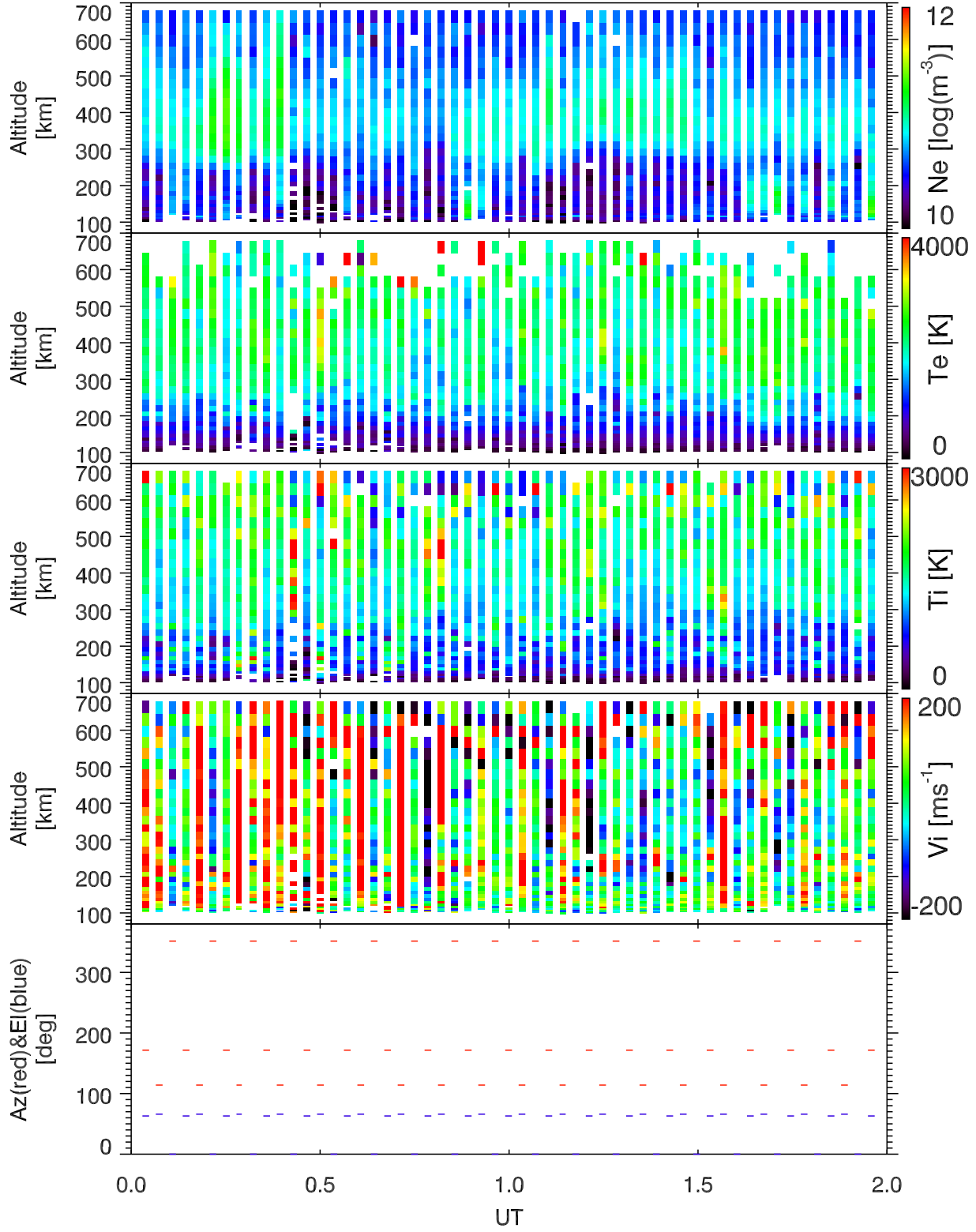
EISCAT 2003-03-22_00_02UT_tau0_ant@32m.
