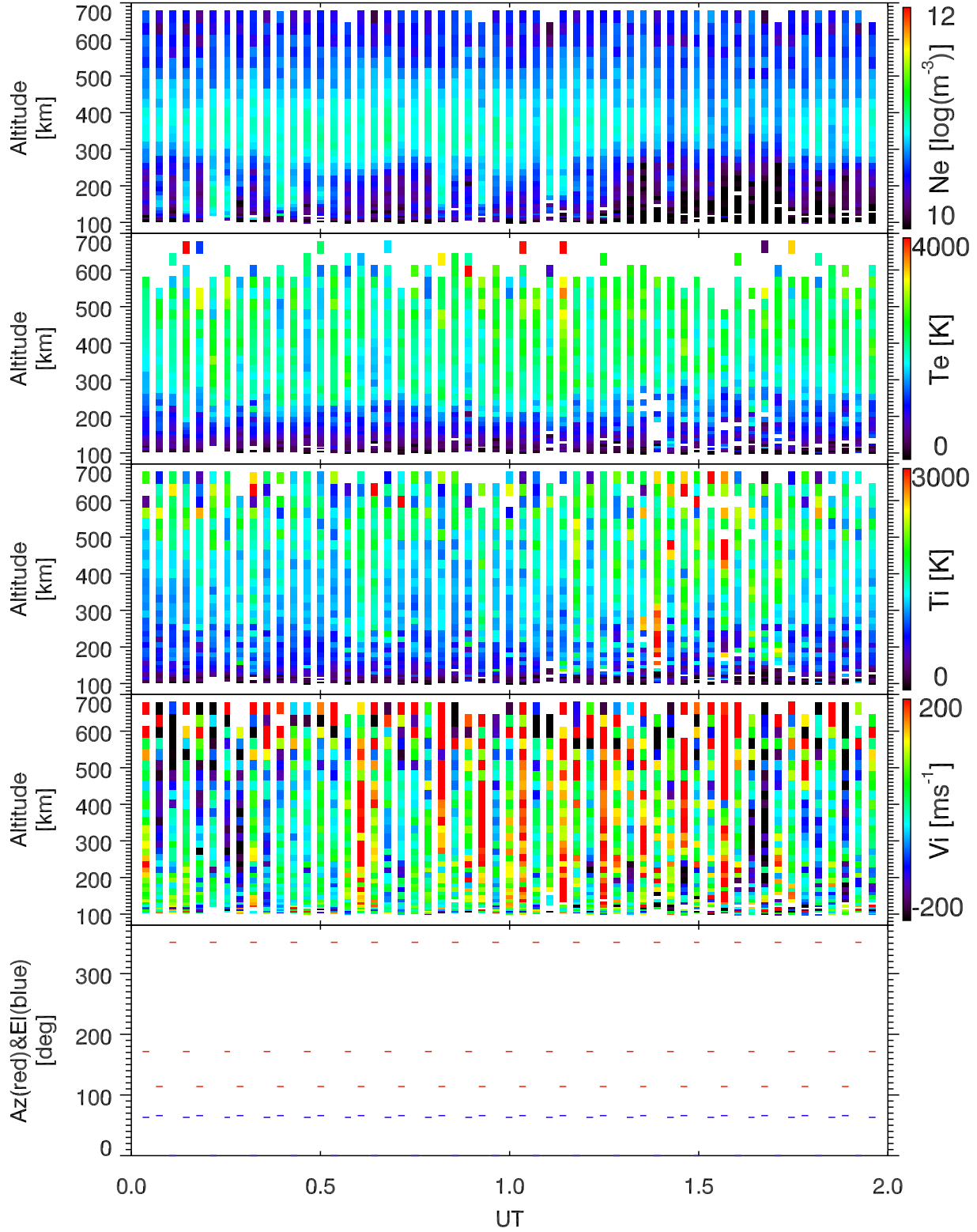
EISCAT 2003-03-23_00_02UT_tau0_ant@32m.
