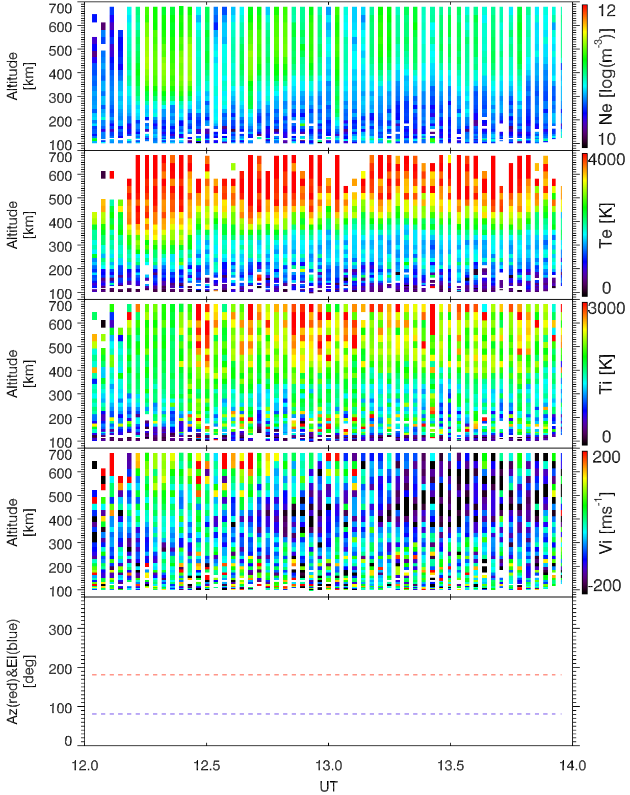
EISCAT 2003-10-29_12_14UT_tau0_ant@42m.
