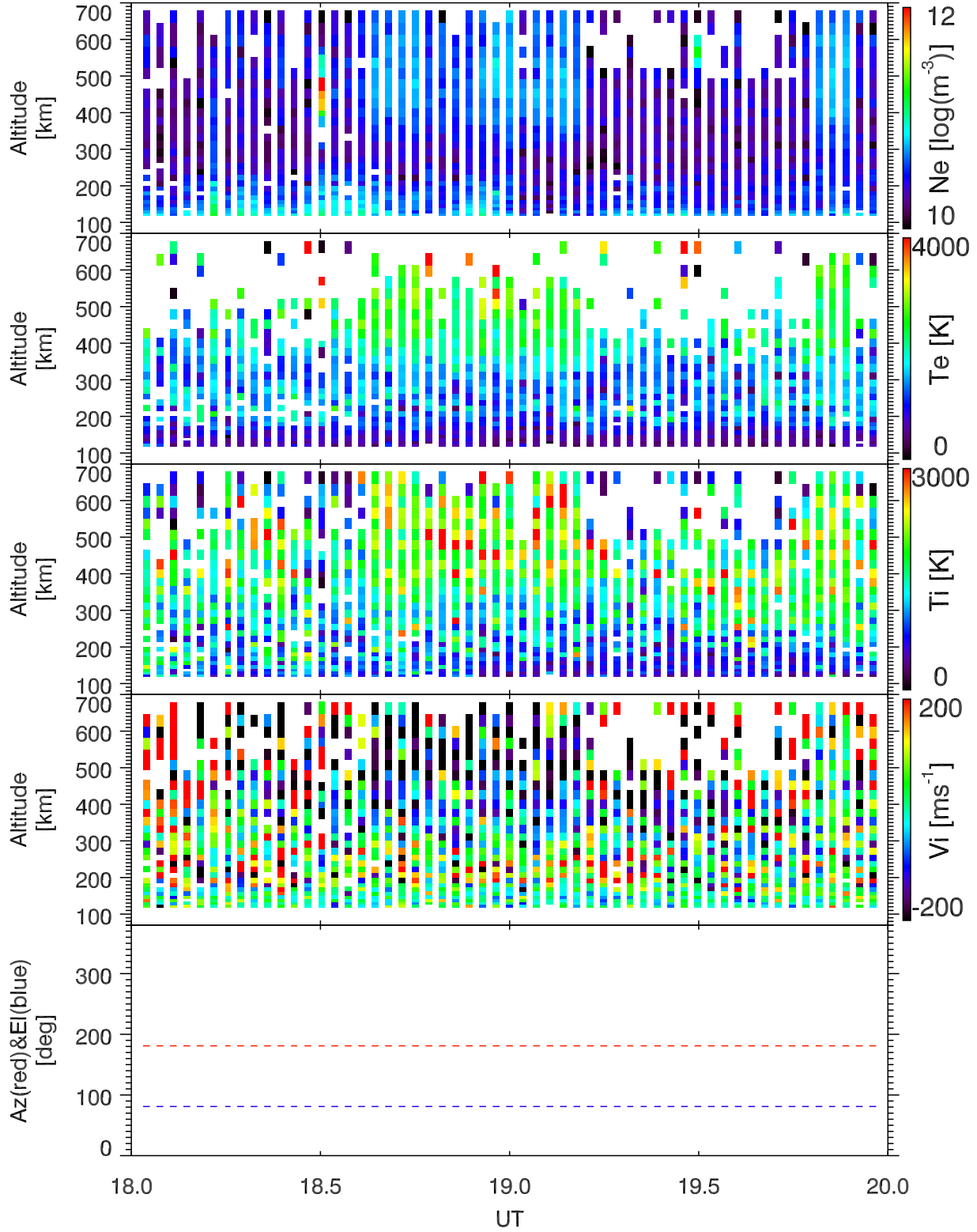
EISCAT 2003-10-29_18_20UT_tau0_ant@42m.
