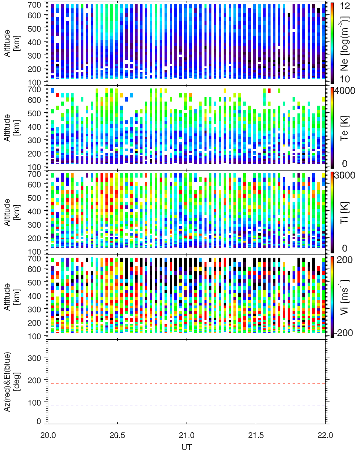
EISCAT 2003-10-29_20_22UT_tau0_ant@42m.
