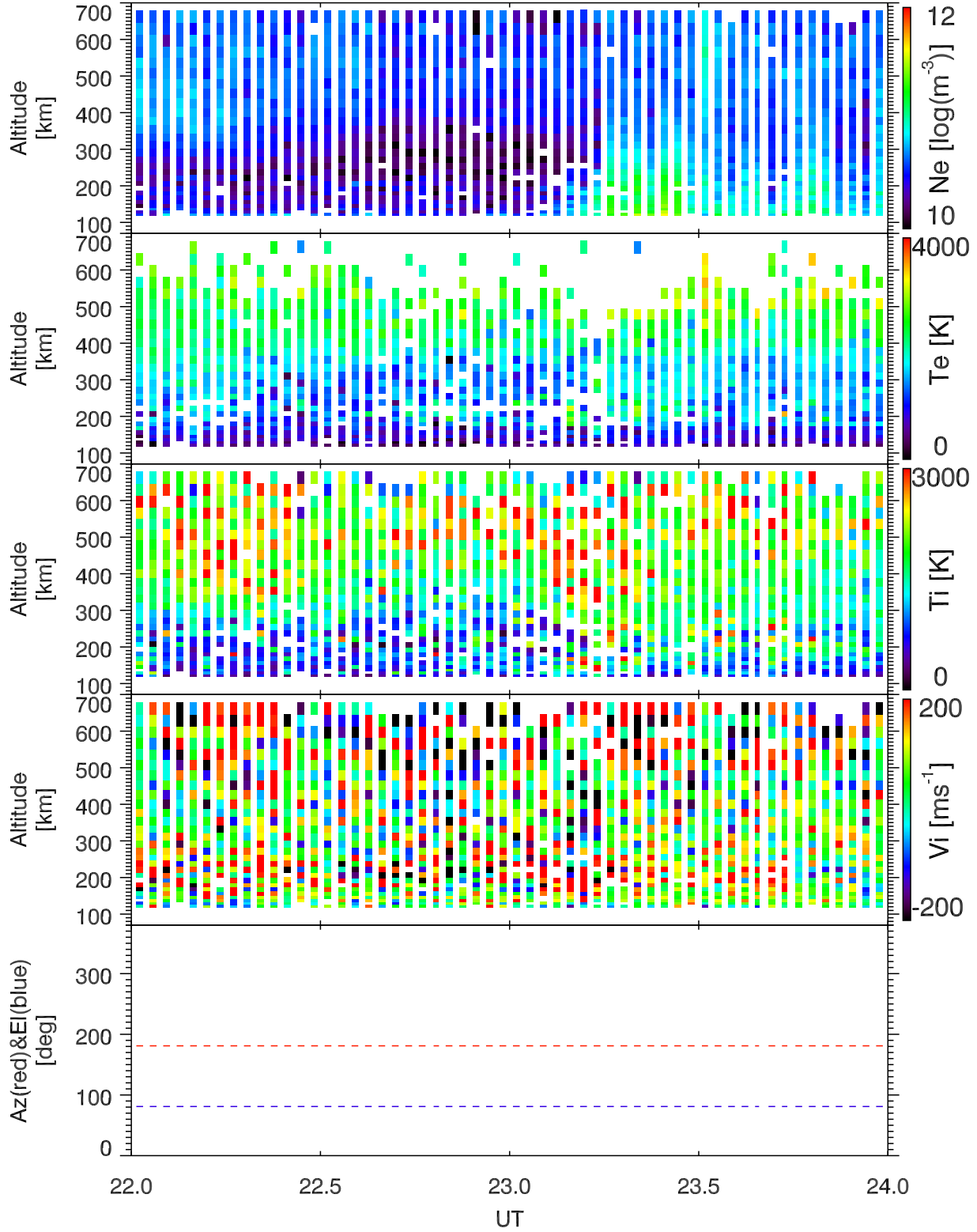
EISCAT 2003-10-29_22_24UT_tau0_ant@42m.
