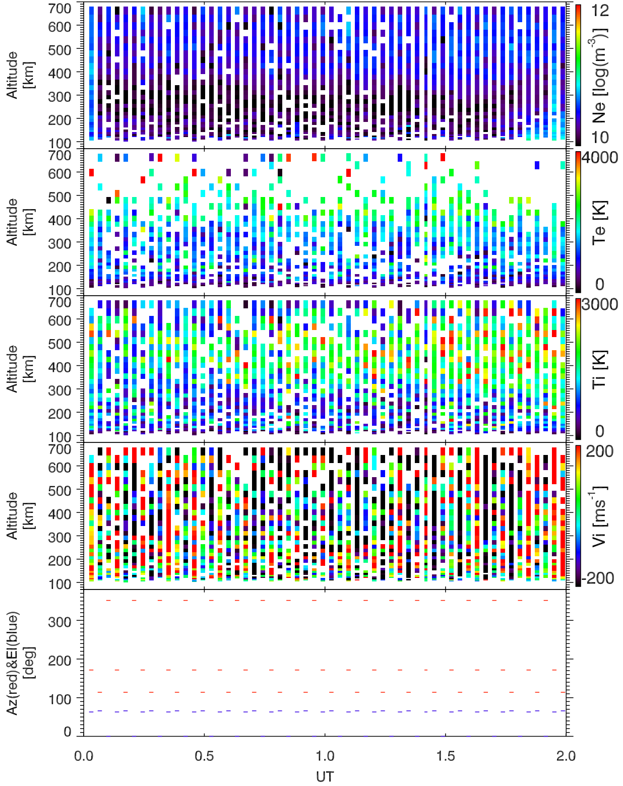
EISCAT 2003-10-30_00_02UT_tau0_ant@32m.
