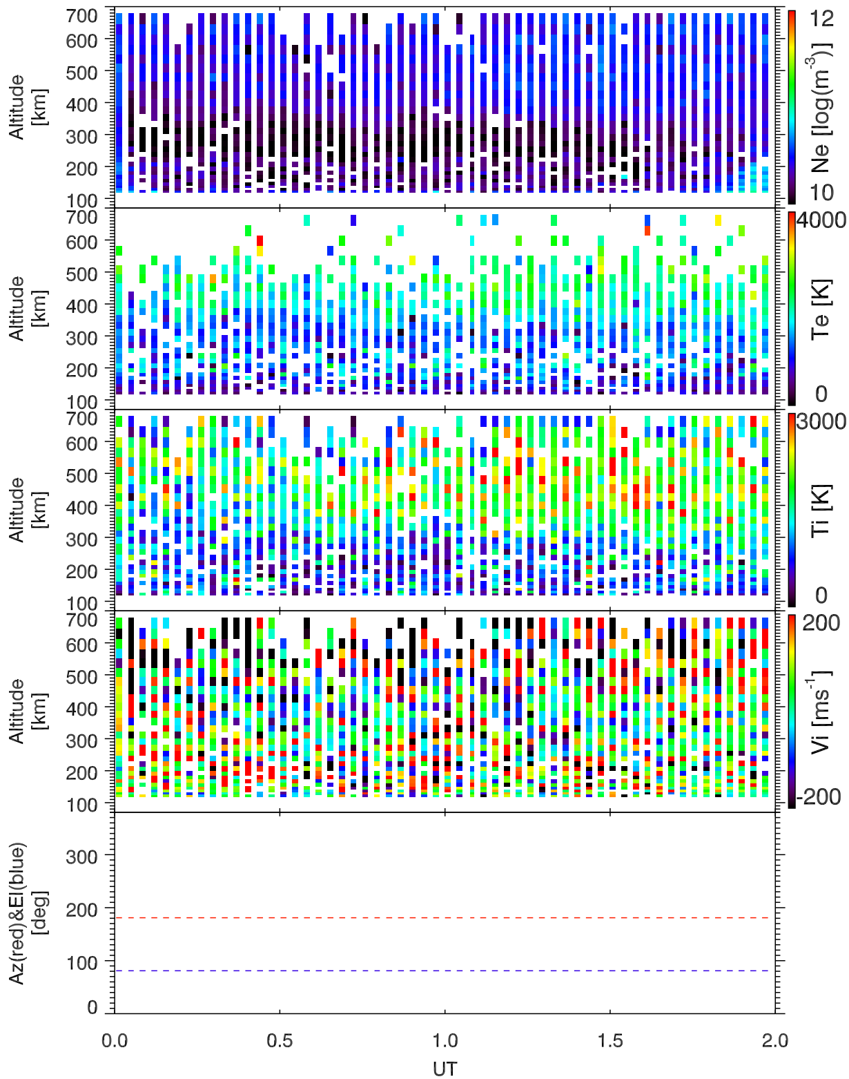
EISCAT 2003-10-30_00_02UT_tau0_ant@42m.
