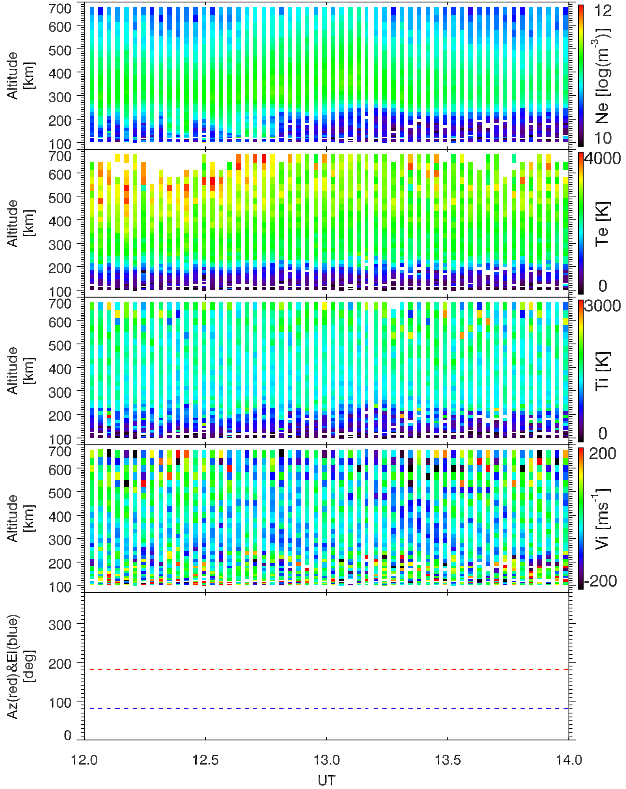
EISCAT 2003-10-30_12_14UT_tau0_ant@42m.
