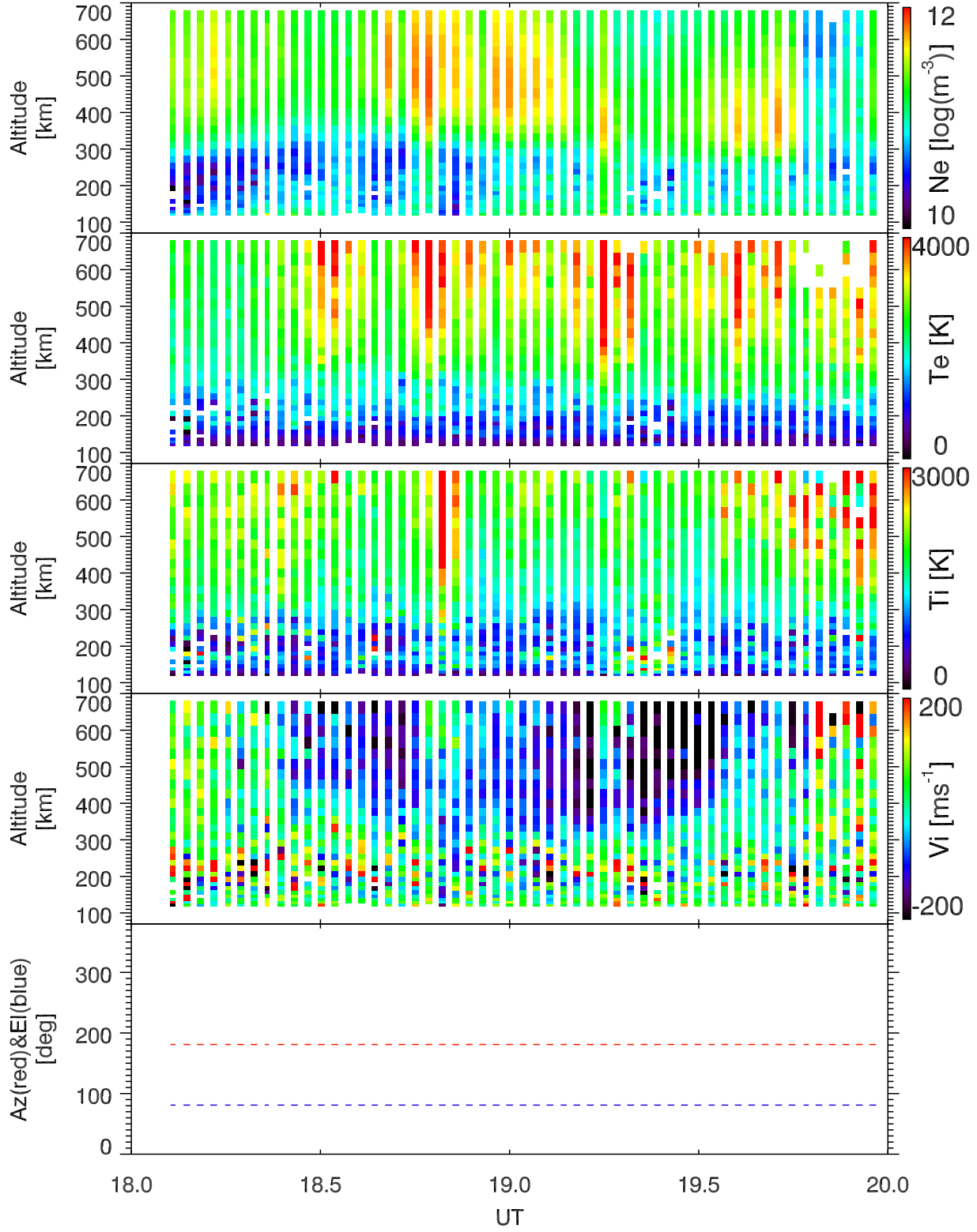
EISCAT 2003-10-30_18_20UT_tau0_ant@42m.
