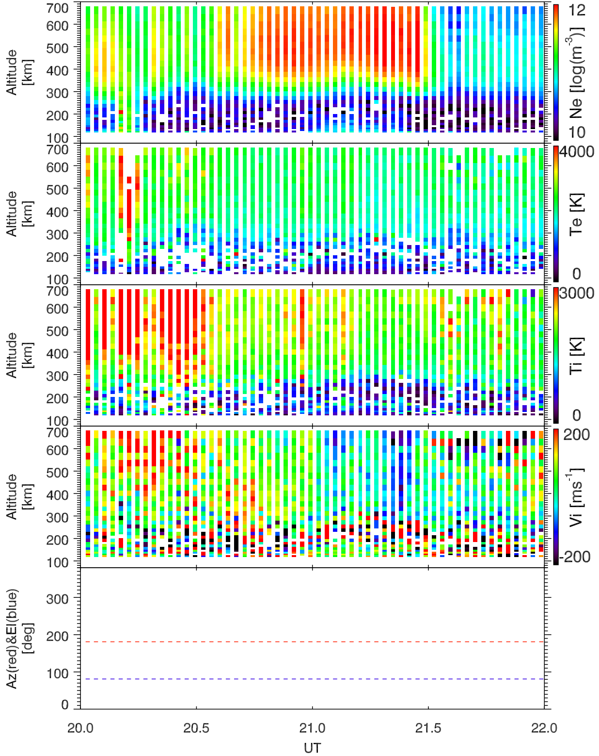
EISCAT 2003-10-30_20_22UT_tau0_ant@42m.
