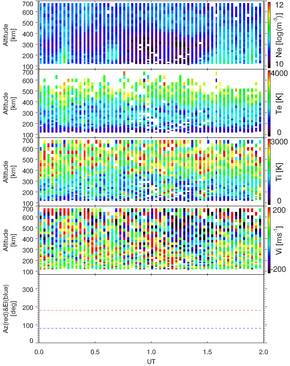
EISCAT 2003-10-31_00_02UT_tau0_ant@42m.
