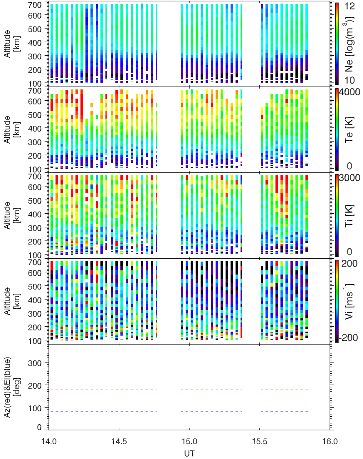
EISCAT 2003-10-31_14_16UT_tau0_ant@42m.
