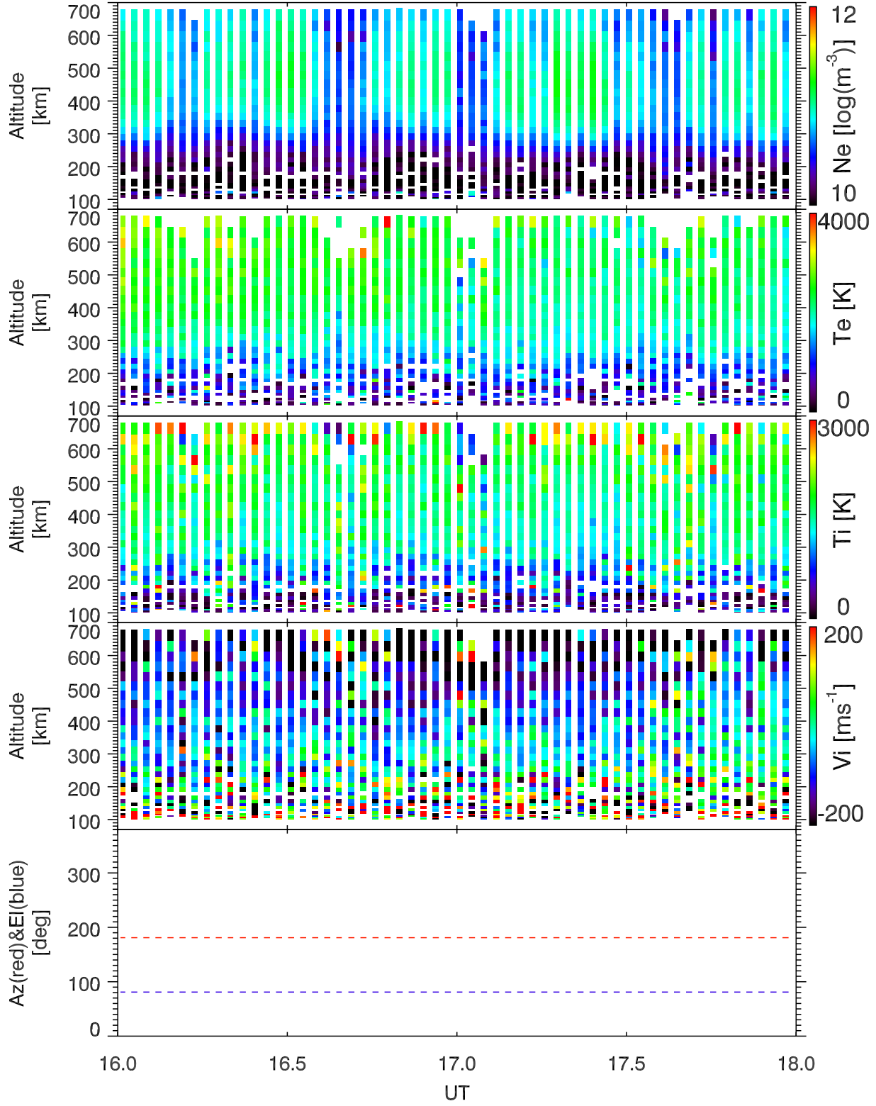
EISCAT 2003-10-31_16_18UT_tau0_ant@42m.
