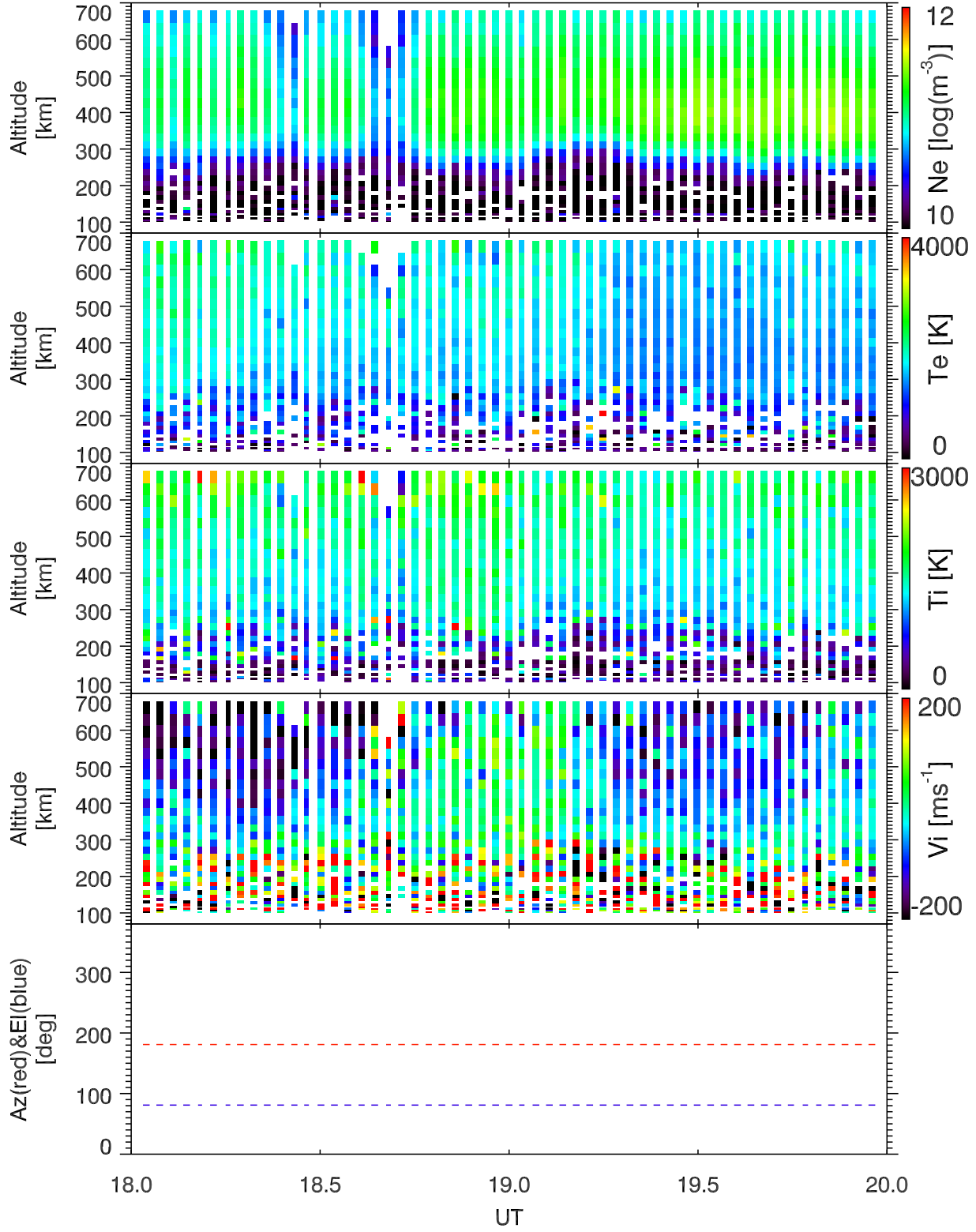
EISCAT 2003-10-31_18_20UT_tau0_ant@42m.
