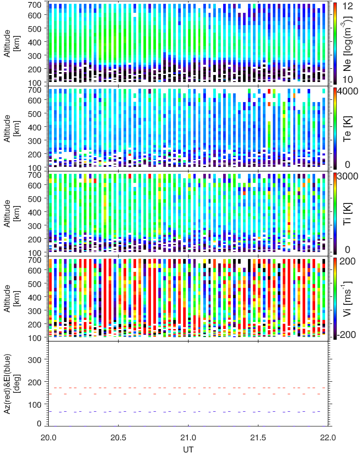
EISCAT 2003-10-31_20_22UT_tau0_ant@32m.
