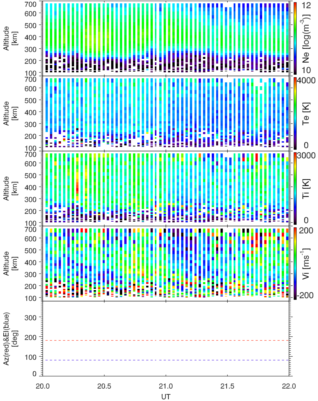
EISCAT 2003-10-31_20_22UT_tau0_ant@42m.
