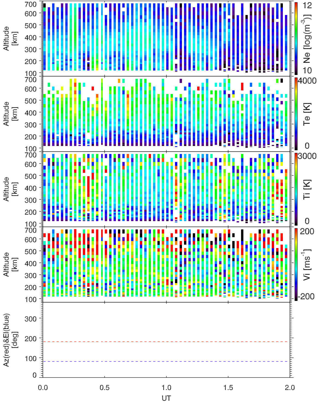
EISCAT 2003-11-01_00_02UT_tau0_ant@42m.
