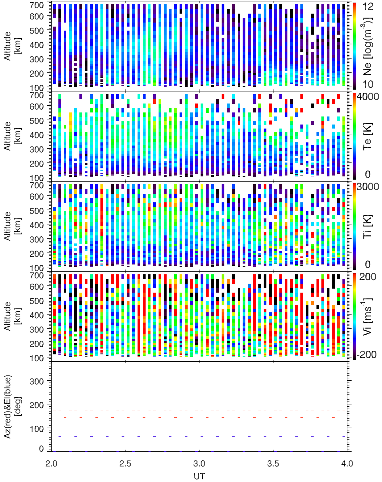
EISCAT 2003-11-01_02_04UT_tau0_ant@32m.
