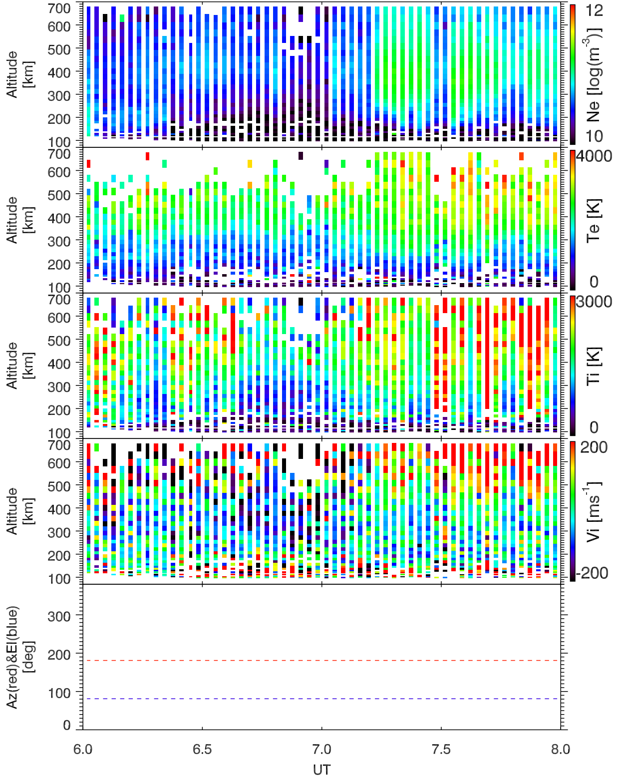
EISCAT 2003-11-01_06_08UT_tau0_ant@42m.
