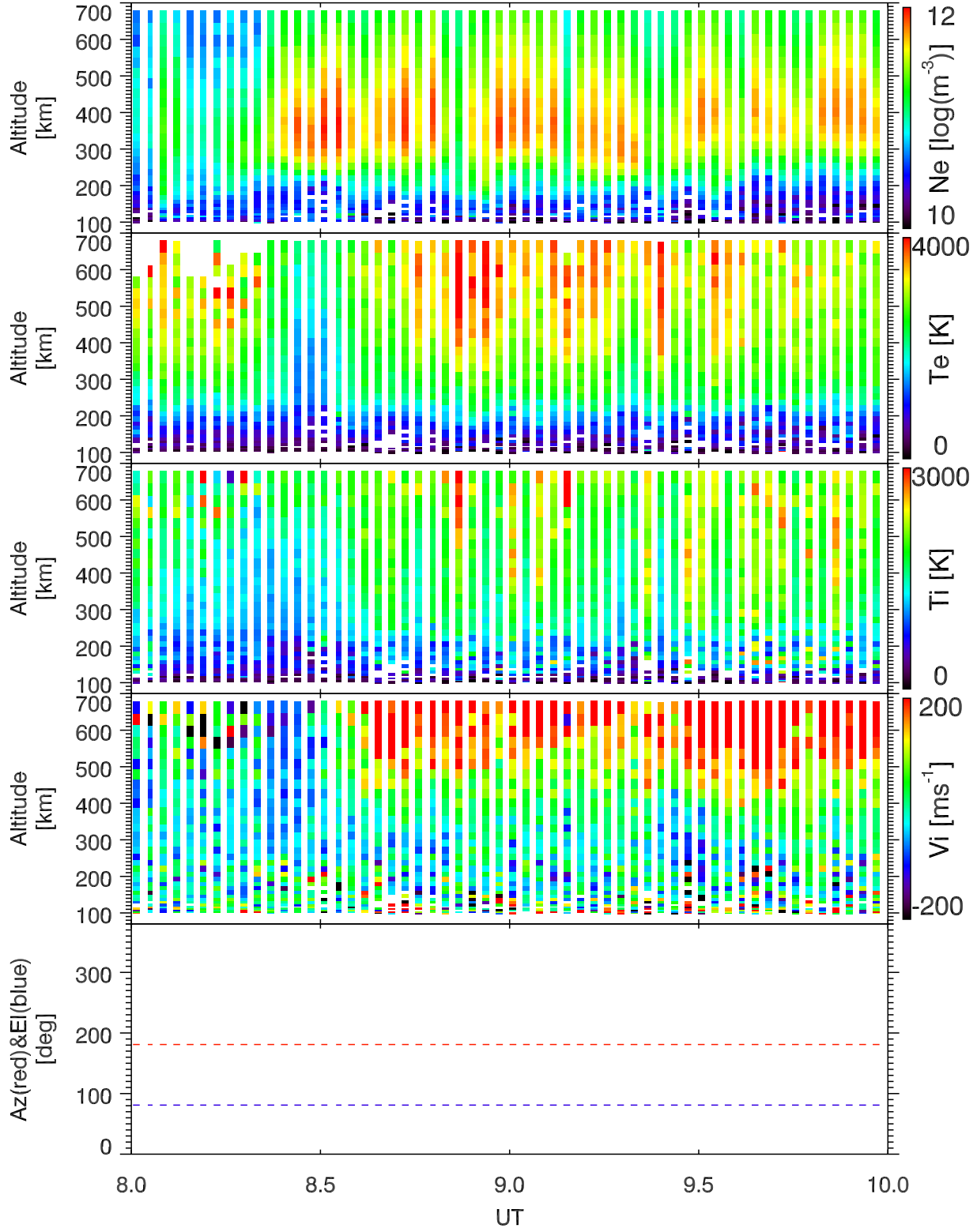
EISCAT 2003-11-01_08_10UT_tau0_ant@42m.
