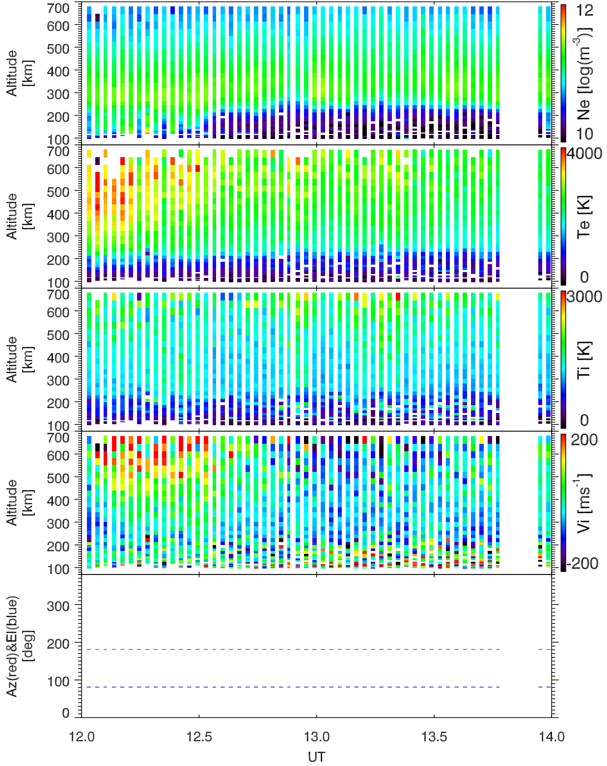
EISCAT 2003-11-01_12_14UT_tau0_ant@42m.
