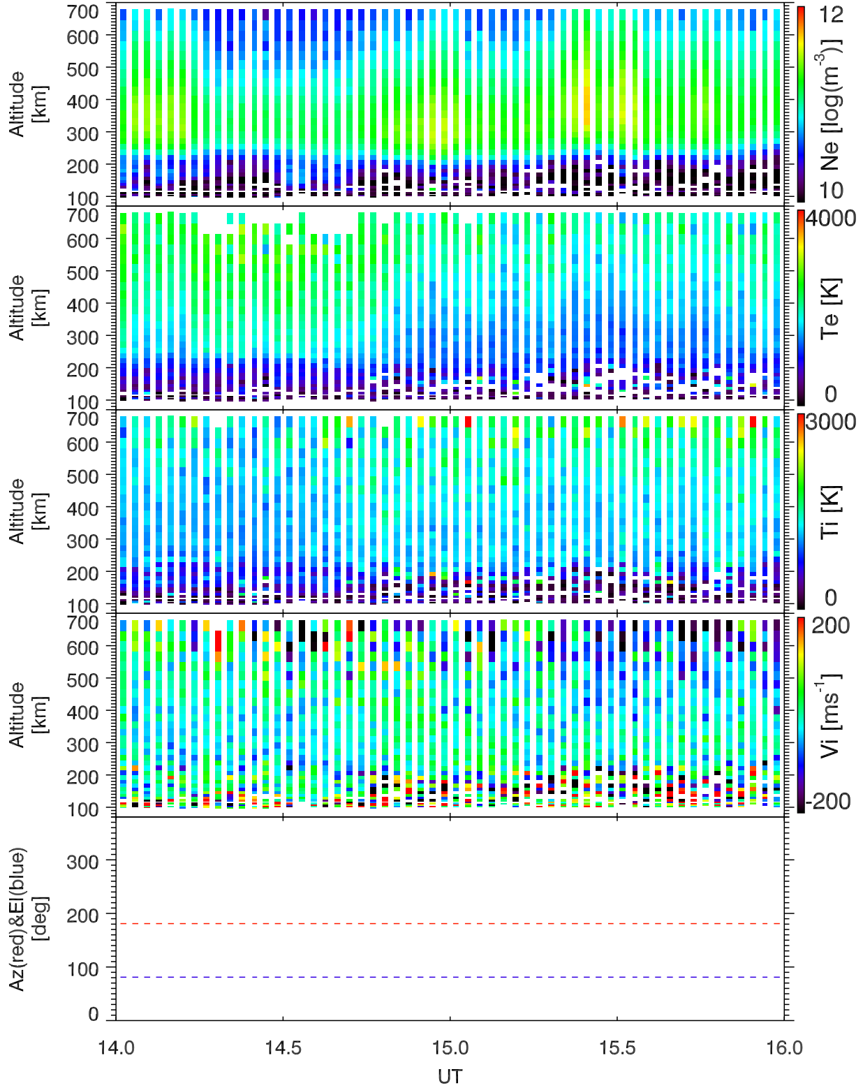
EISCAT 2003-11-01_14_16UT_tau0_ant@42m.
