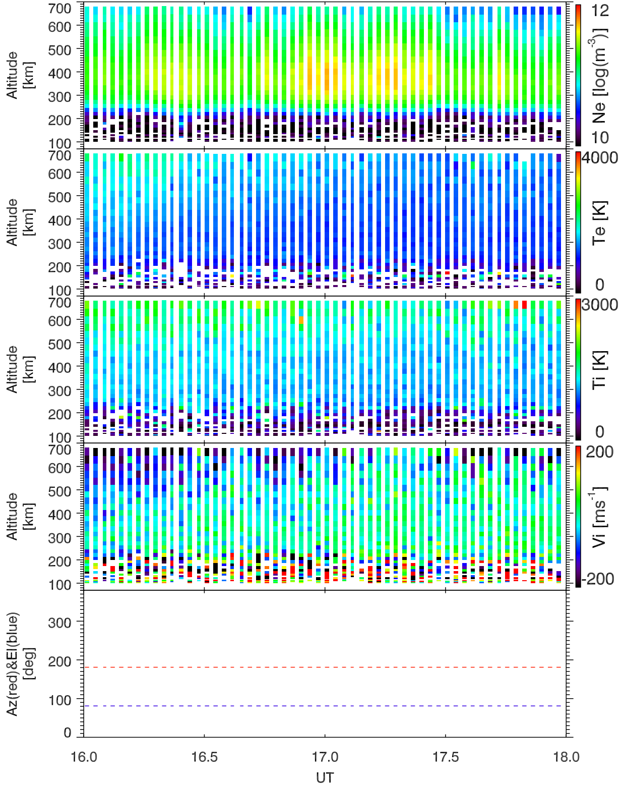
EISCAT 2003-11-01_16_18UT_tau0_ant@42m.
