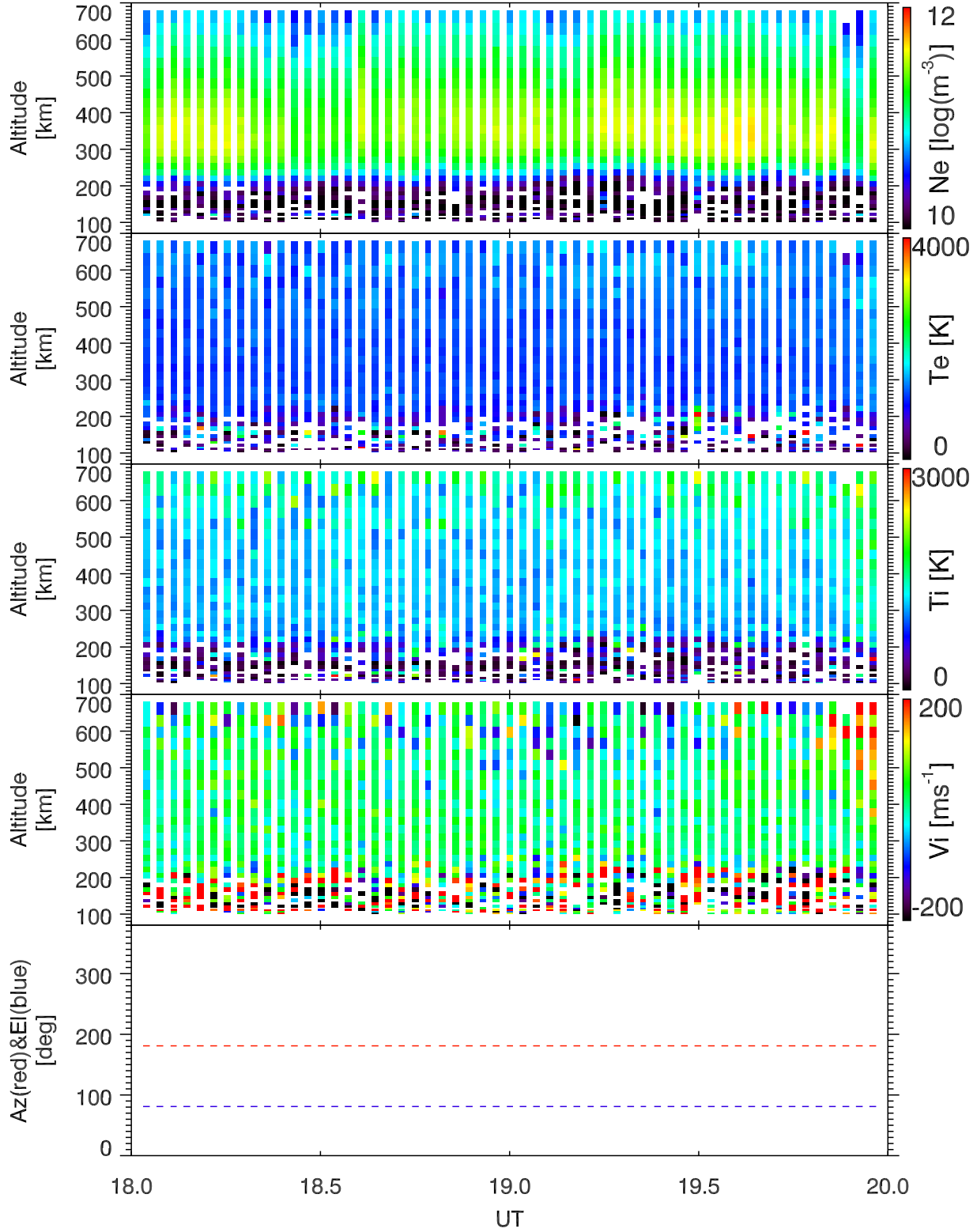
EISCAT 2003-11-01_18_20UT_tau0_ant@42m.
