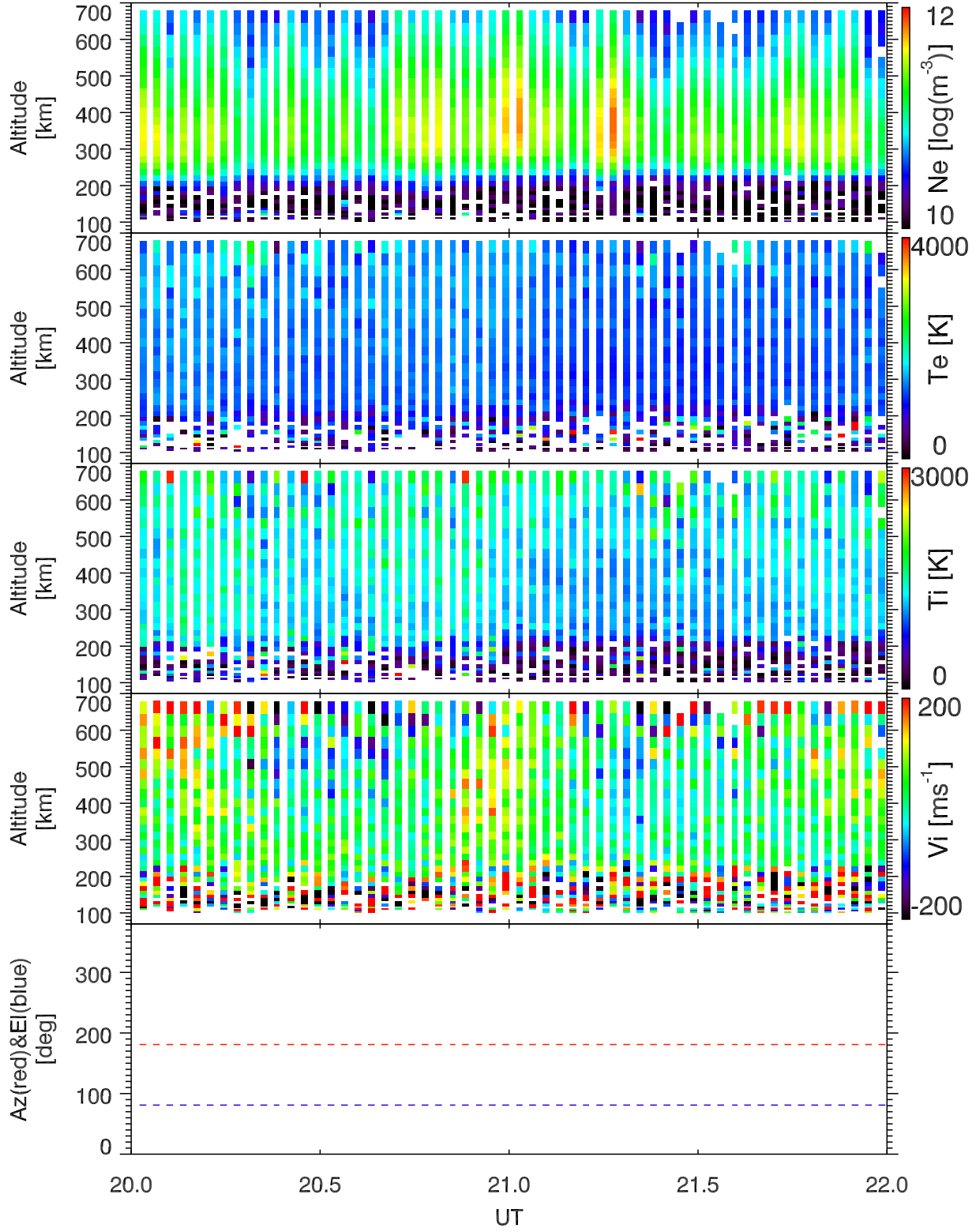
EISCAT 2003-11-01_20_22UT_tau0_ant@42m.
