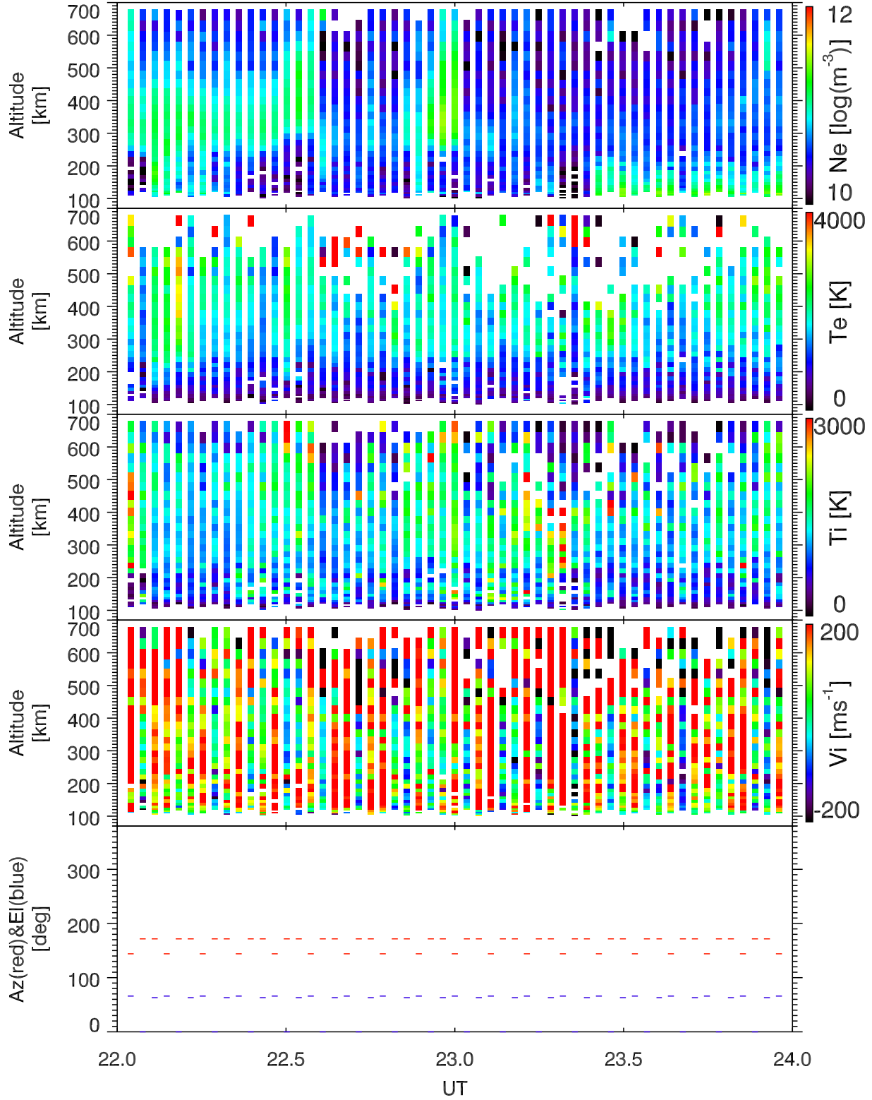
EISCAT 2003-11-01_22_24UT_tau0_ant@32m.
