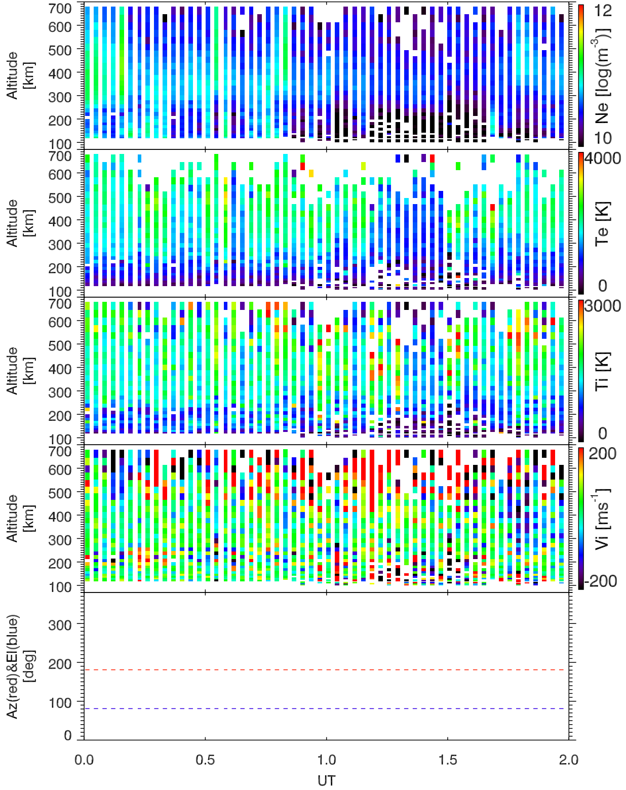
EISCAT 2003-11-02_00_02UT_tau0_ant@42m.
