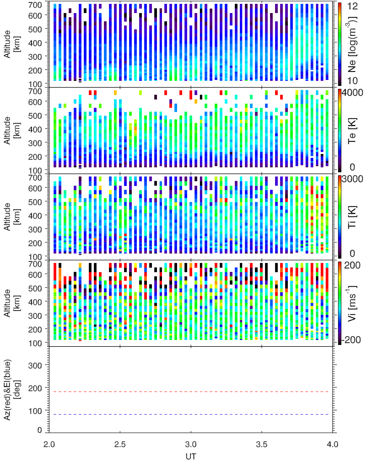
EISCAT 2003-11-02_02_04UT_tau0_ant@42m.
