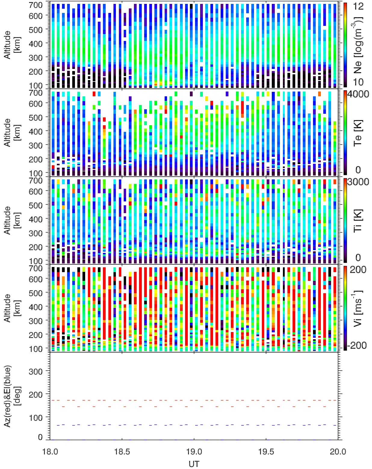
EISCAT 2003-11-13_18_20UT_steffe_ant@32m.
