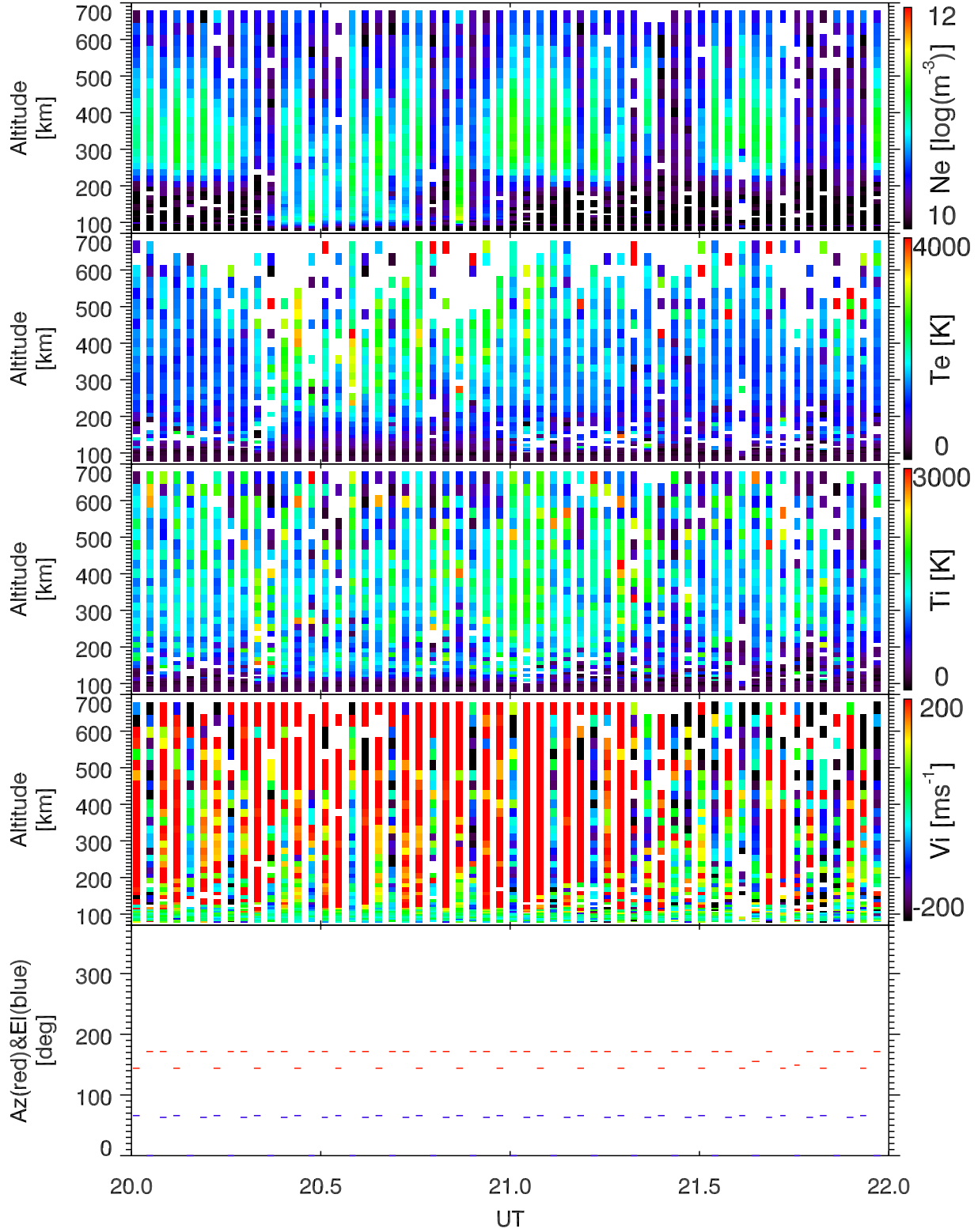
EISCAT 2003-11-14_20_22UT_steffe_ant@32m.
