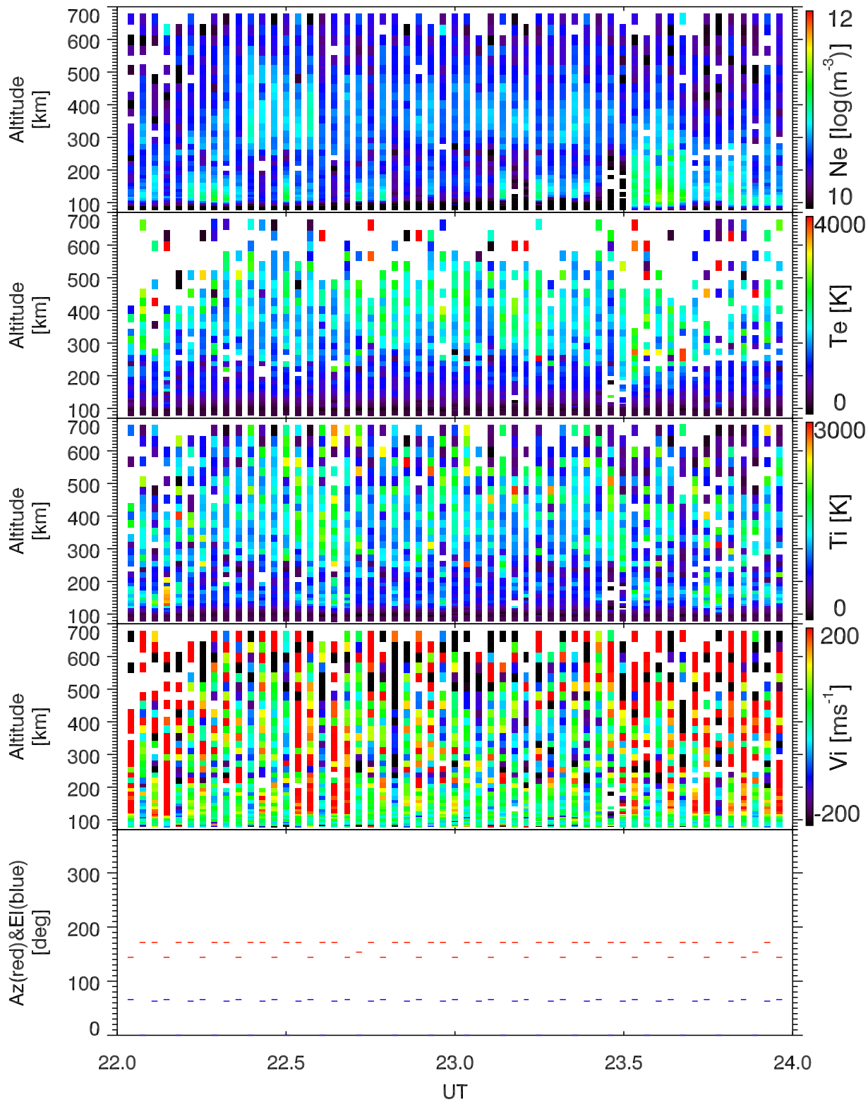
EISCAT 2003-11-15_22_24UT_steffe_ant@32m.
