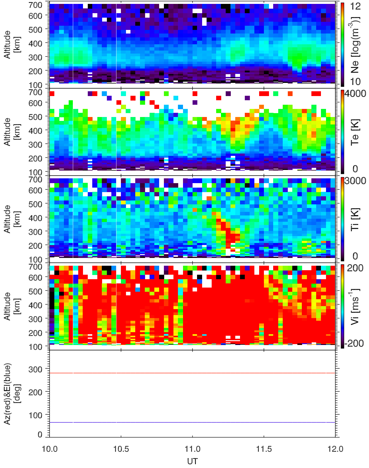
EISCAT 2003-11-27_10_12UT_tau0_120@32m.
