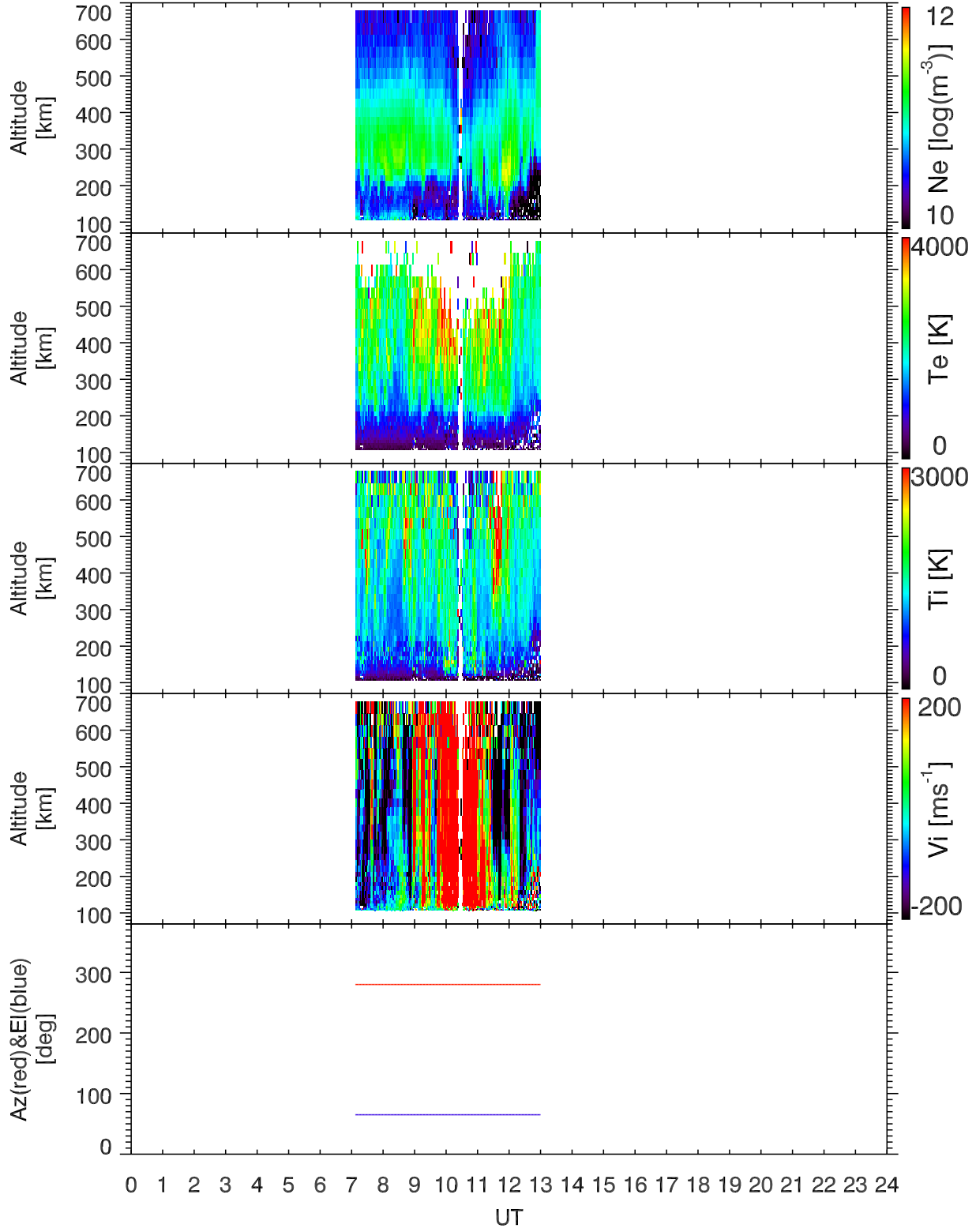
EISCAT 2003-11-28_00_24UT_tau0_120@32m.
